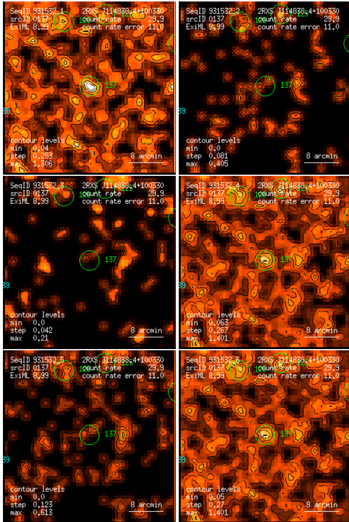
Figure 137: RASS 931532: detection 0137: band rate images, Gaussian filter: (1) PSPC channels 11 – 41, (2) 52 – 90, (3) 91 – 201, (4) 11 – 235, (5) 52 – 201, (6) 11 – 201. Broad band rates in counts/ks. Band rate contour levels in counts/ks/arcmin 2 .
