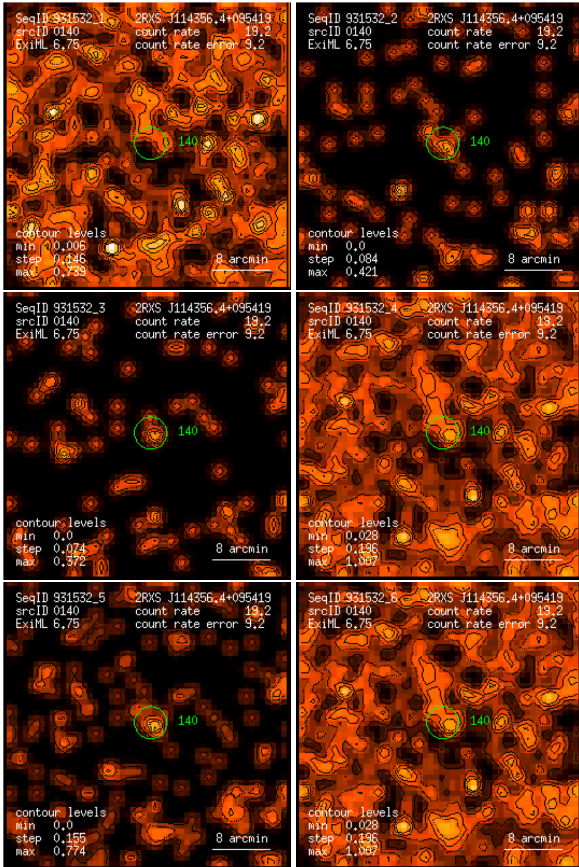
Figure 140: RASS 931532: detection 0140: band rate images, Gaussian filter: (1) PSPC channels 11 – 41, (2) 52 – 90, (3) 91 – 201, (4) 11 – 235, (5) 52 – 201, (6) 11 – 201. Broad band rates in counts/ks. Band rate contour levels in counts/ks/arcmin 2 .
