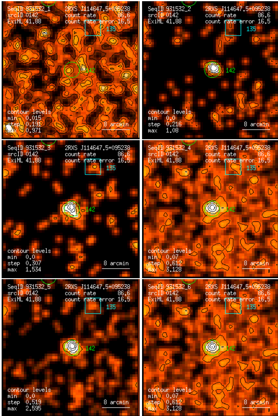
Figure 142: RASS 931532: detection 0142: band rate images, Gaussian filter: (1) PSPC channels 11 – 41, (2) 52 – 90, (3) 91 – 201, (4) 11 – 235, (5) 52 – 201, (6) 11 – 201. Broad band rates in counts/ks. Band rate contour levels in counts/ks/arcmin 2 .
