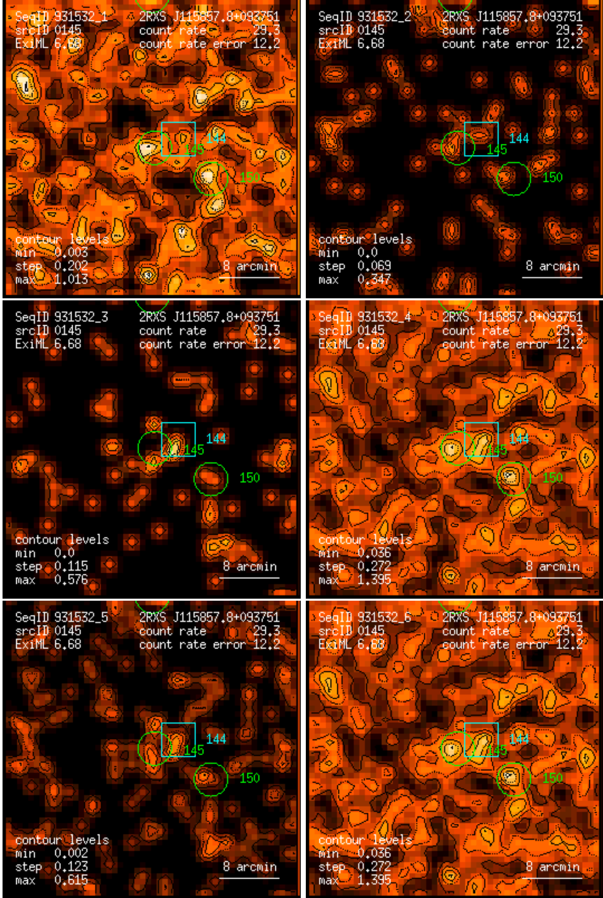
Figure 145: RASS 931532: detection 0145: band rate images, Gaussian filter: (1) PSPC channels 11 – 41, (2) 52 – 90, (3) 91 – 201, (4) 11 – 235, (5) 52 – 201, (6) 11 – 201. Broad band rates in counts/ks. Band rate contour levels in counts/ks/arcmin 2 .
