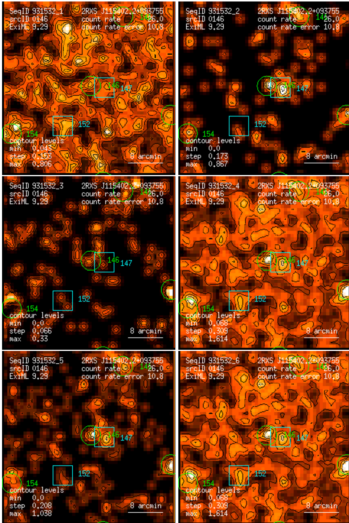
Figure 146: RASS 931532: detection 0146: band rate images, Gaussian filter: (1) PSPC channels 11 – 41, (2) 52 – 90, (3) 91 – 201, (4) 11 – 235, (5) 52 – 201, (6) 11 – 201. Broad band rates in counts/ks. Band rate contour levels in counts/ks/arcmin 2 .
