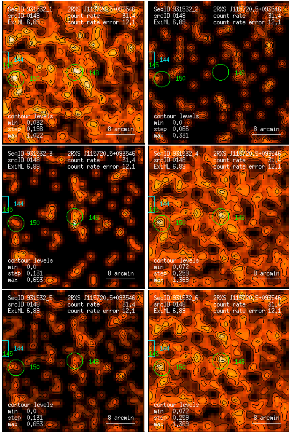
Figure 148: RASS 931532: detection 0148: band rate images, Gaussian filter: (1) PSPC channels 11 – 41, (2) 52 – 90, (3) 91 – 201, (4) 11 – 235, (5) 52 – 201, (6) 11 – 201. Broad band rates in counts/ks. Band rate contour levels in counts/ks/arcmin 2 .
