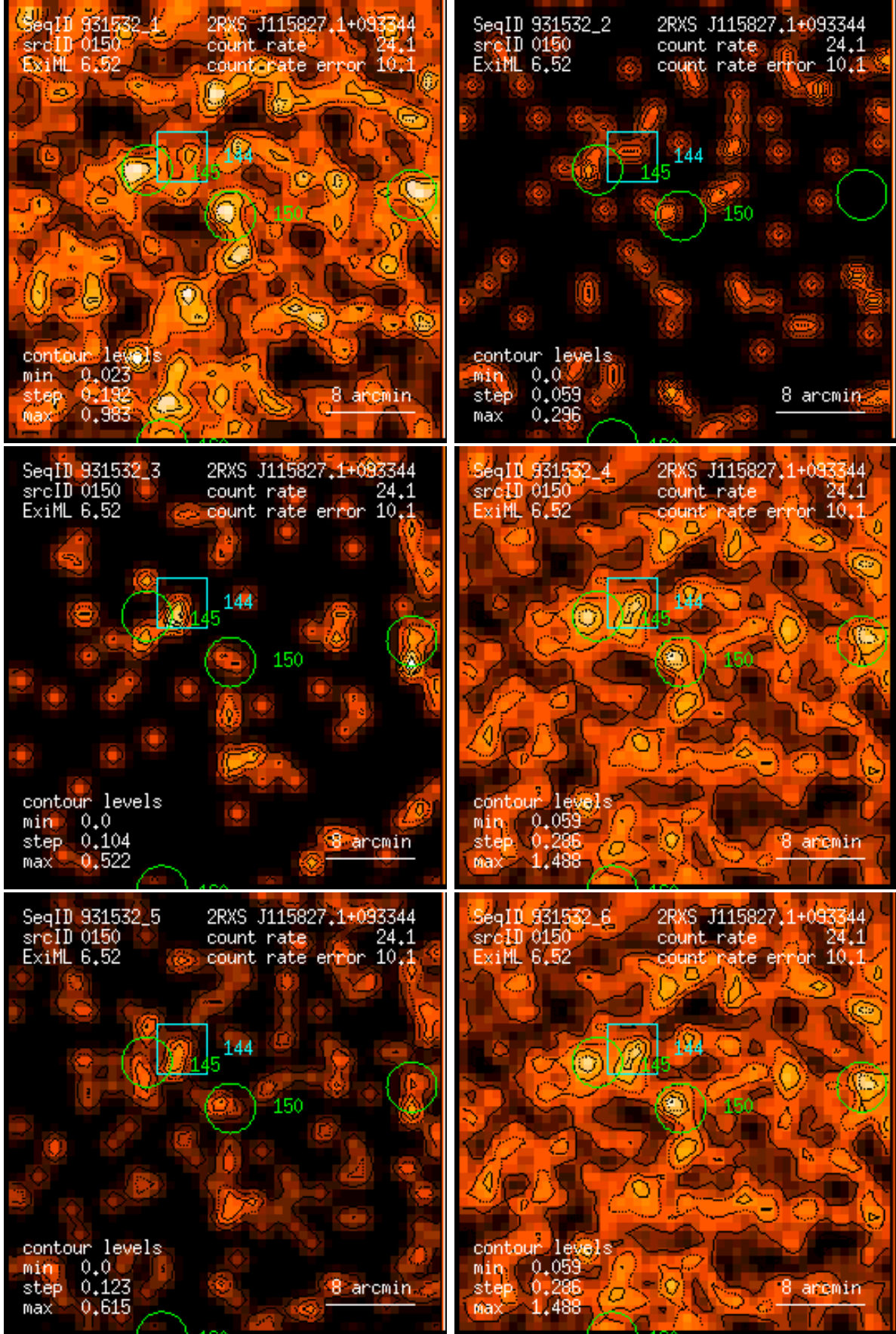
Figure 150: RASS 931532: detection 0150: band rate images, Gaussian filter: (1) PSPC channels 11 – 41, (2) 52 – 90, (3) 91 – 201, (4) 11 – 235, (5) 52 – 201, (6) 11 – 201. Broad band rates in counts/ks. Band rate contour levels in counts/ks/arcmin 2 .
