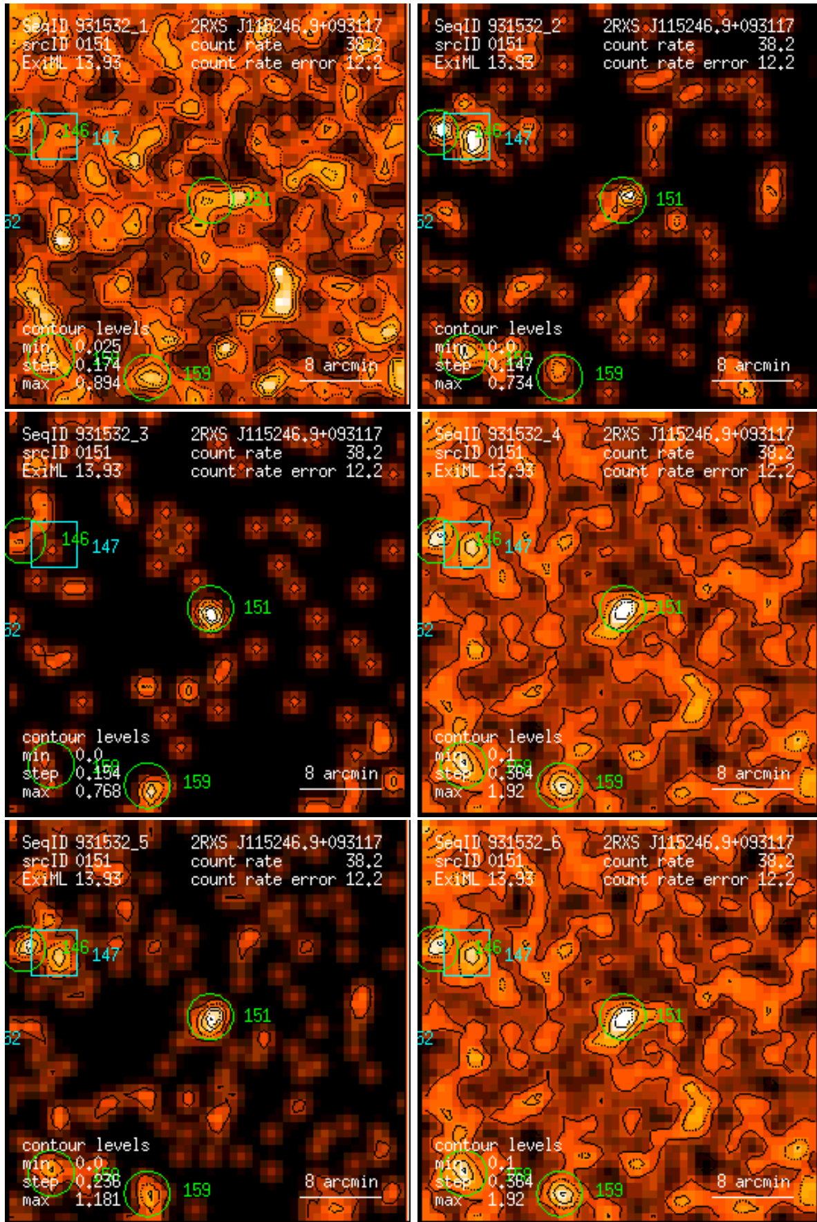
Figure 151: RASS 931532: detection 0151: band rate images, Gaussian filter: (1) PSPC channels 11 – 41, (2) 52 – 90, (3) 91 – 201, (4) 11 – 235, (5) 52 – 201, (6) 11 – 201. Broad band rates in counts/ks. Band rate contour levels in counts/ks/arcmin 2 .
