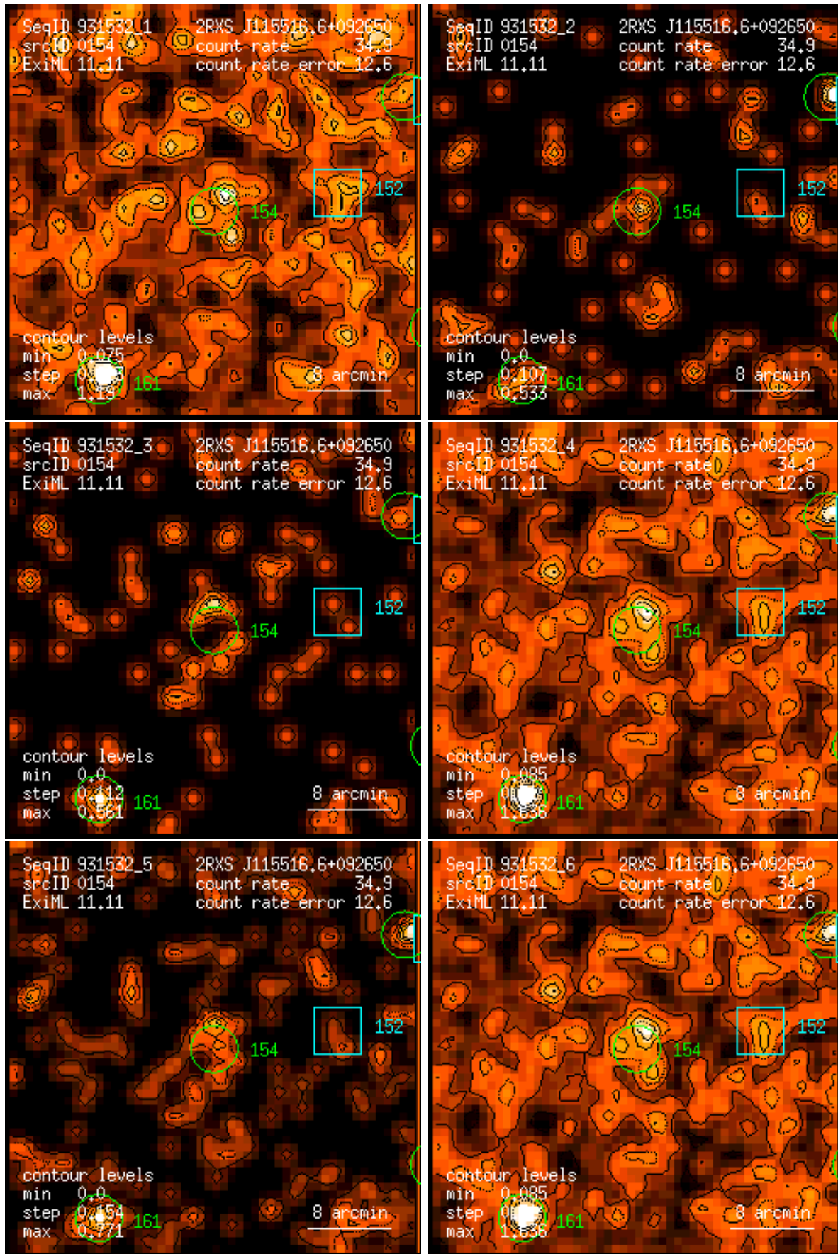
Figure 154: RASS 931532: detection 0154: band rate images, Gaussian filter: (1) PSPC channels 11 – 41, (2) 52 – 90, (3) 91 – 201, (4) 11 – 235, (5) 52 – 201, (6) 11 – 201. Broad band rates in counts/ks. Band rate contour levels in counts/ks/arcmin 2 .
