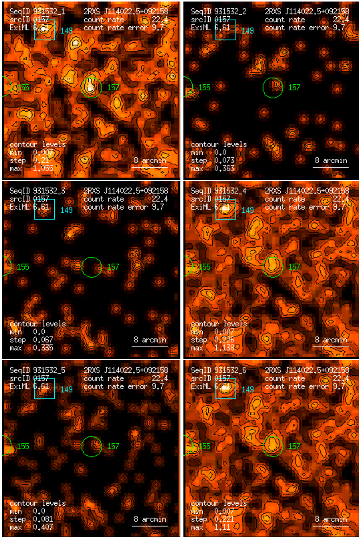
Figure 157: RASS 931532: detection 0157: band rate images, Gaussian filter: (1) PSPC channels 11 – 41, (2) 52 – 90, (3) 91 – 201, (4) 11 – 235, (5) 52 – 201, (6) 11 – 201. Broad band rates in counts/ks. Band rate contour levels in counts/ks/arcmin 2 .
