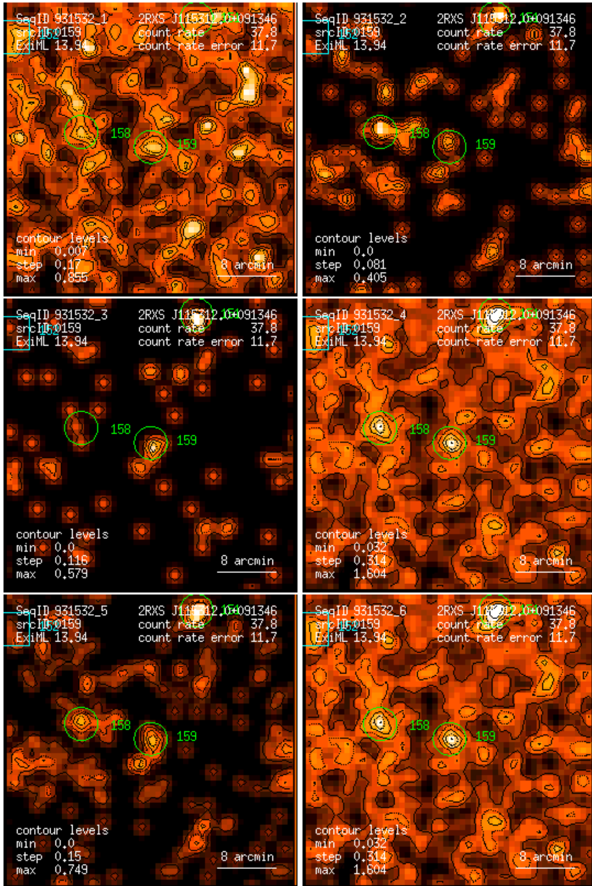
Figure 159: RASS 931532: detection 0159: band rate images, Gaussian filter: (1) PSPC channels 11 – 41, (2) 52 – 90, (3) 91 – 201, (4) 11 – 235, (5) 52 – 201, (6) 11 – 201. Broad band rates in counts/ks. Band rate contour levels in counts/ks/arcmin 2 .
