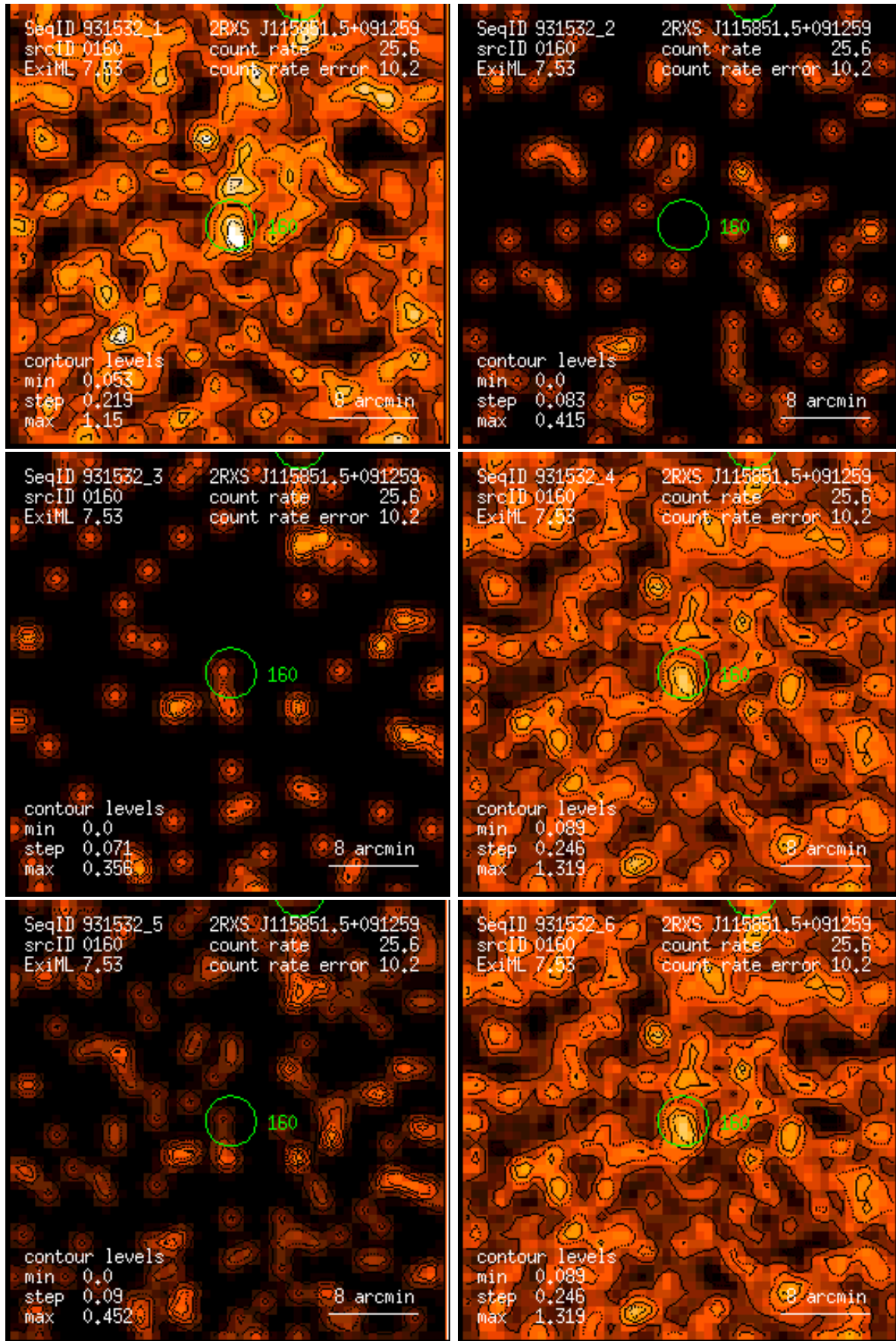
Figure 160: RASS 931532: detection 0160: band rate images, Gaussian filter: (1) PSPC channels 11 – 41, (2) 52 – 90, (3) 91 – 201, (4) 11 – 235, (5) 52 – 201, (6) 11 – 201. Broad band rates in counts/ks. Band rate contour levels in counts/ks/arcmin 2 .
