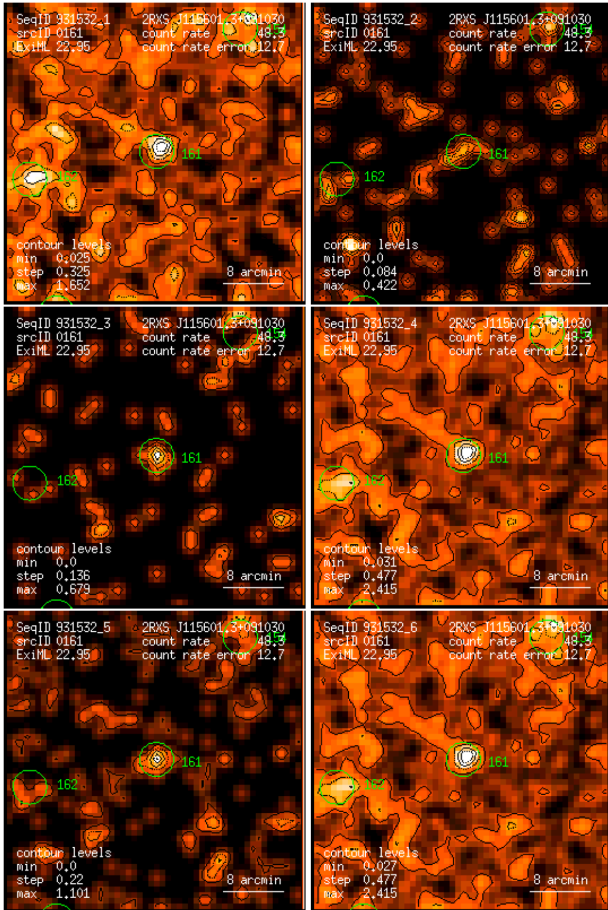
Figure 161: RASS 931532: detection 0161: band rate images, Gaussian filter: (1) PSPC channels 11 – 41, (2) 52 – 90, (3) 91 – 201, (4) 11 – 235, (5) 52 – 201, (6) 11 – 201. Broad band rates in counts/ks. Band rate contour levels in counts/ks/arcmin 2 .
