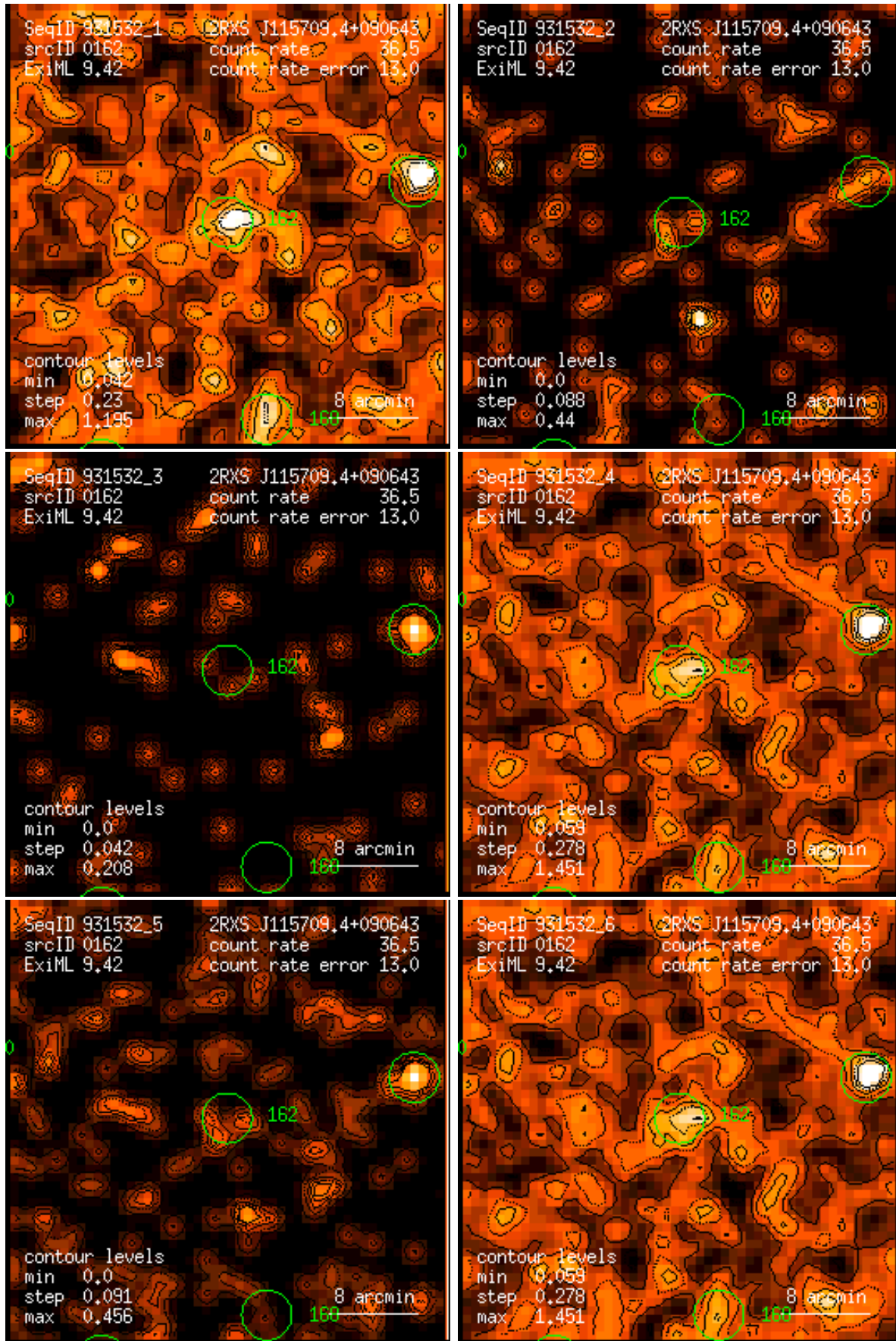
Figure 162: RASS 931532: detection 0162: band rate images, Gaussian filter: (1) PSPC channels 11 – 41, (2) 52 – 90, (3) 91 – 201, (4) 11 – 235, (5) 52 – 201, (6) 11 – 201. Broad band rates in counts/ks. Band rate contour levels in counts/ks/arcmin 2 .
