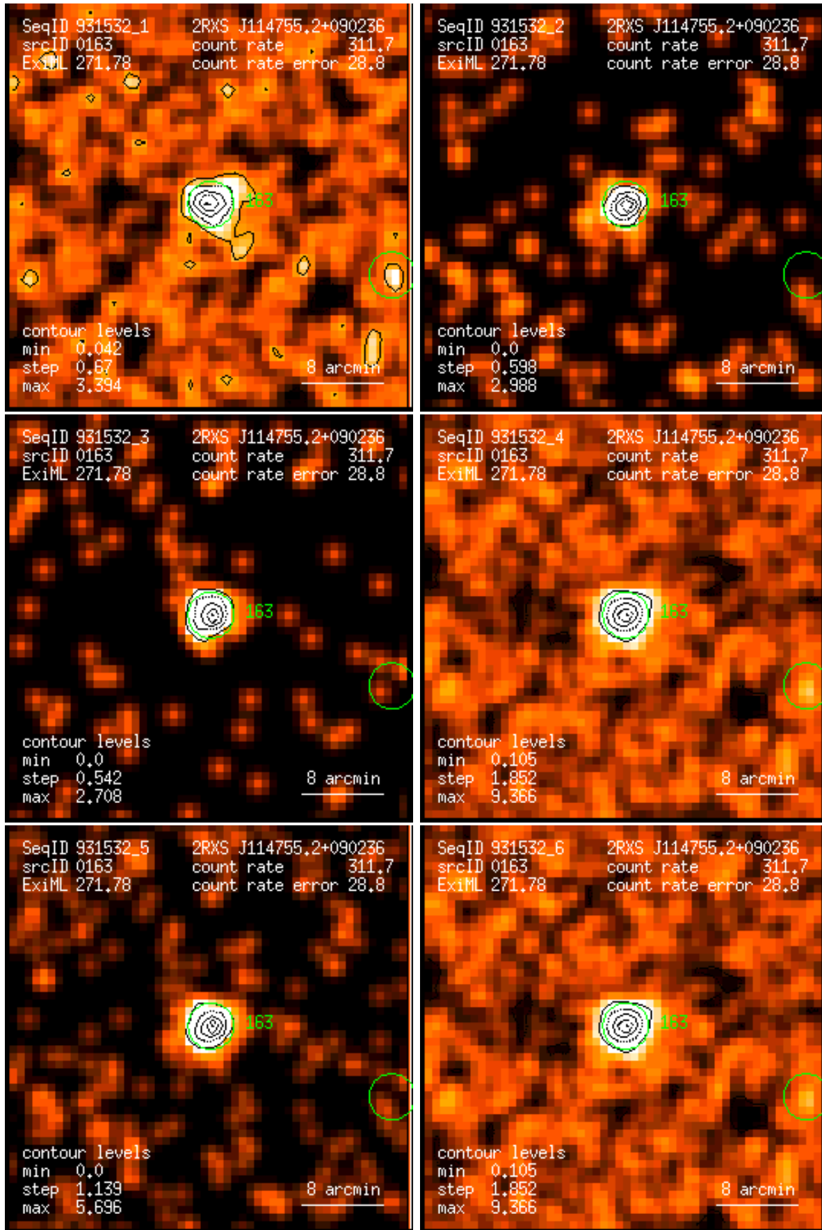
Figure 163: RASS 931532: detection 0163: band rate images, Gaussian filter: (1) PSPC channels 11 – 41, (2) 52 – 90, (3) 91 – 201, (4) 11 – 235, (5) 52 – 201, (6) 11 – 201. Broad band rates in counts/ks. Band rate contour levels in counts/ks/arcmin 2 .
