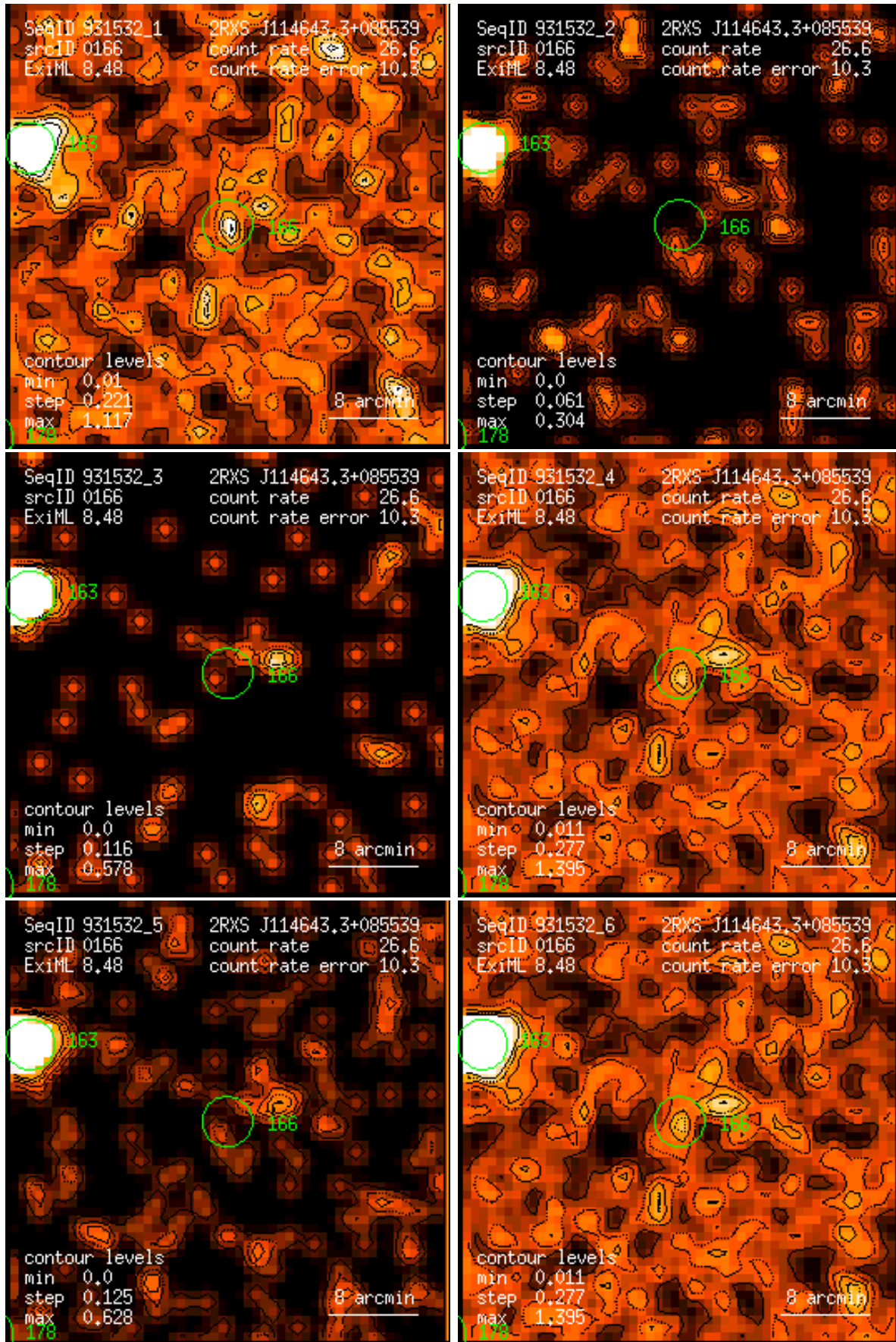
Figure 166: RASS 931532: detection 0166: band rate images, Gaussian filter: (1) PSPC channels 11 – 41, (2) 52 – 90, (3) 91 – 201, (4) 11 – 235, (5) 52 – 201, (6) 11 – 201. Broad band rates in counts/ks. Band rate contour levels in counts/ks/arcmin 2 .
