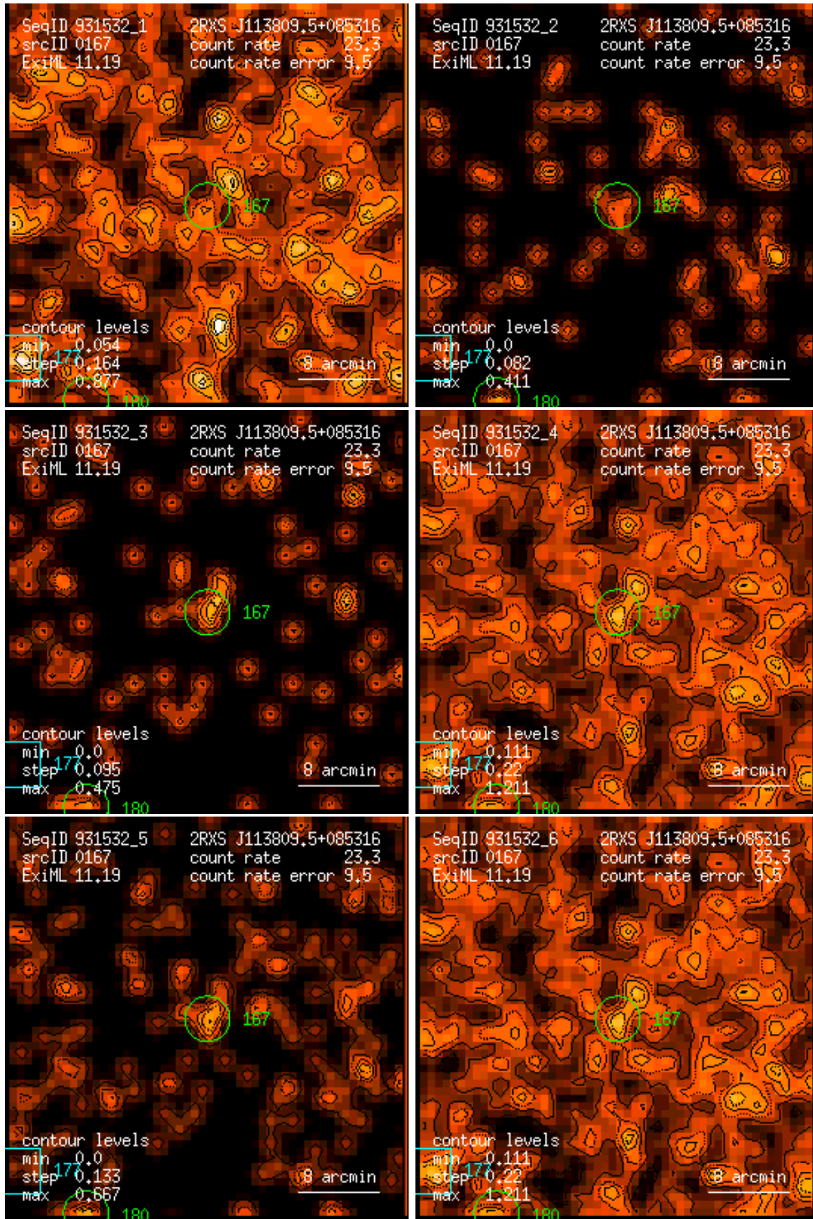
Figure 167: RASS 931532: detection 0167: band rate images, Gaussian filter: (1) PSPC channels 11 – 41, (2) 52 – 90, (3) 91 – 201, (4) 11 – 235, (5) 52 – 201, (6) 11 – 201. Broad band rates in counts/ks. Band rate contour levels in counts/ks/arcmin 2 .
