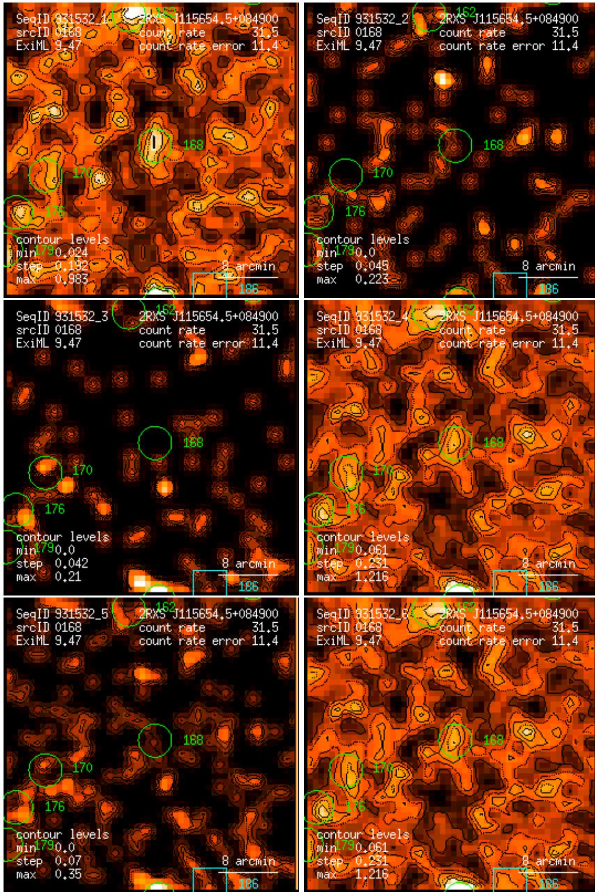
Figure 168: RASS 931532: detection 0168: band rate images, Gaussian filter: (1) PSPC channels 11 – 41, (2) 52 – 90, (3) 91 – 201, (4) 11 – 235, (5) 52 – 201, (6) 11 – 201. Broad band rates in counts/ks. Band rate contour levels in counts/ks/arcmin 2 .
