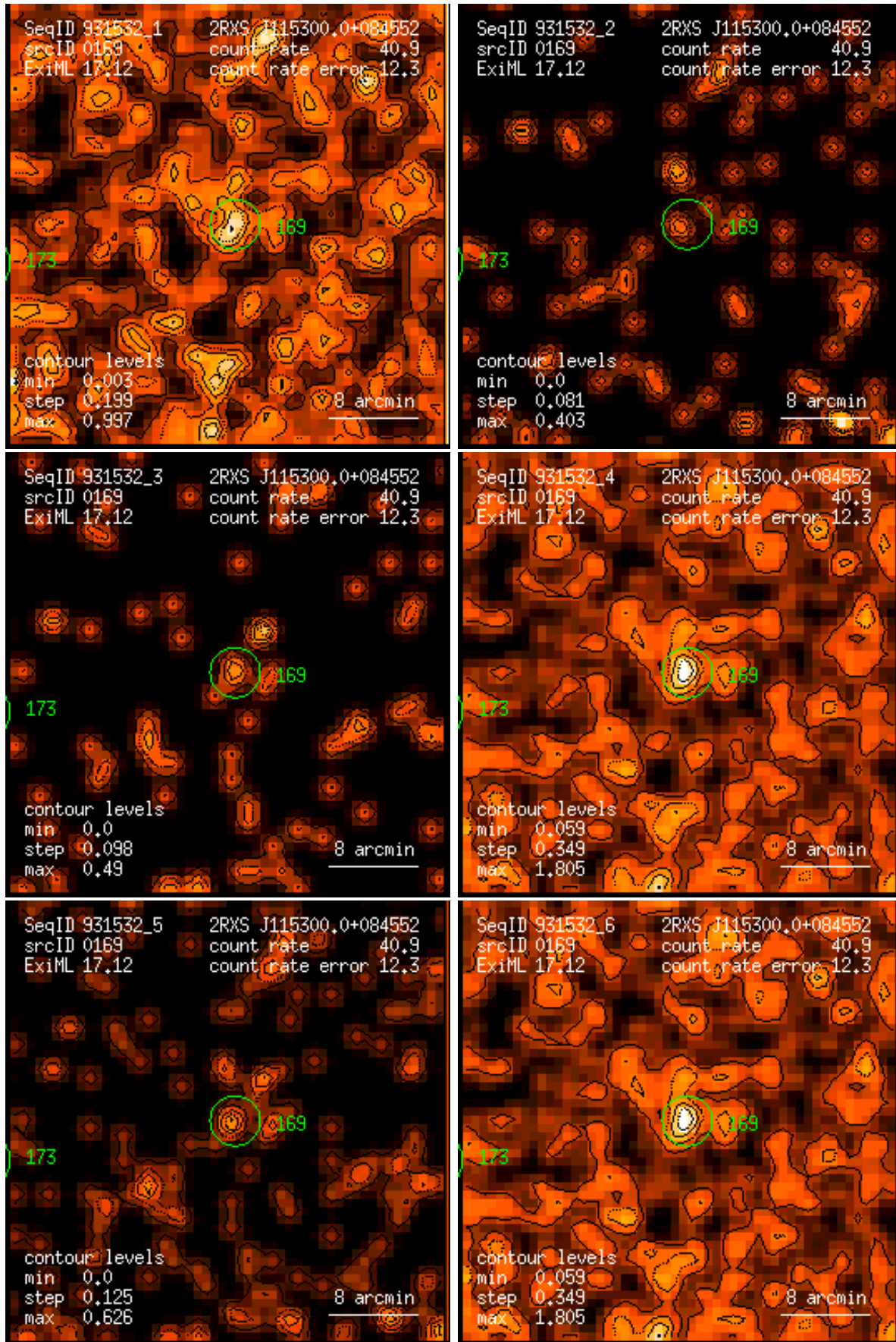
Figure 169: RASS 931532: detection 0169: band rate images, Gaussian filter: (1) PSPC channels 11 – 41, (2) 52 – 90, (3) 91 – 201, (4) 11 – 235, (5) 52 – 201, (6) 11 – 201. Broad band rates in counts/ks. Band rate contour levels in counts/ks/arcmin 2 .
