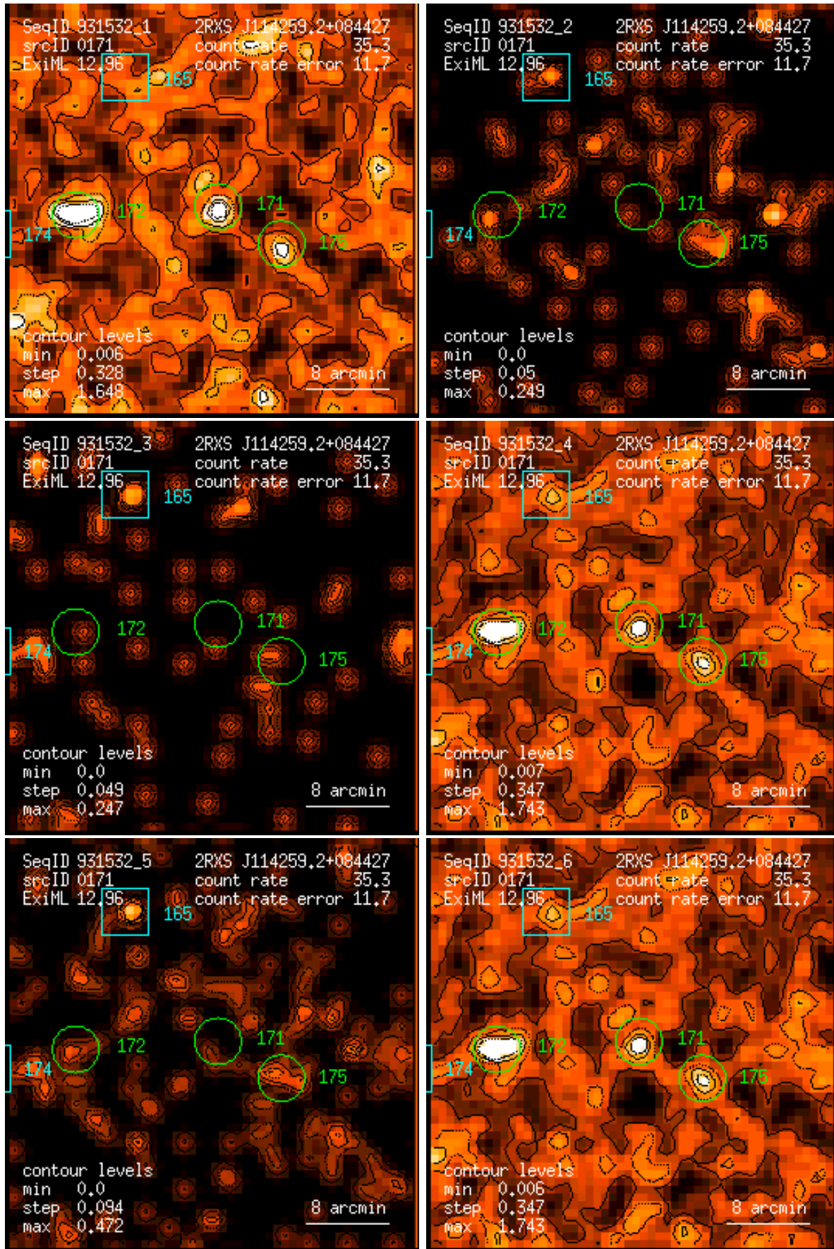
Figure 171: RASS 931532: detection 0171: band rate images, Gaussian filter: (1) PSPC channels 11 – 41, (2) 52 – 90, (3) 91 – 201, (4) 11 – 235, (5) 52 – 201, (6) 11 – 201. Broad band rates in counts/ks. Band rate contour levels in counts/ks/arcmin 2 .
