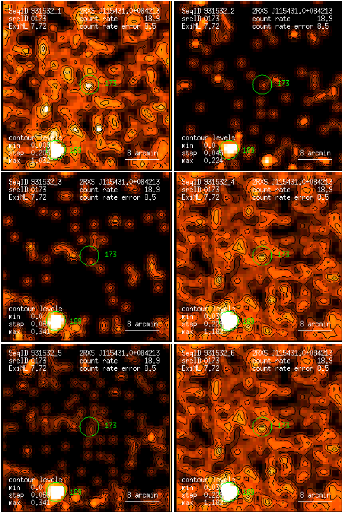
Figure 173: RASS 931532: detection 0173: band rate images, Gaussian filter: (1) PSPC channels 11 – 41, (2) 52 – 90, (3) 91 – 201, (4) 11 – 235, (5) 52 – 201, (6) 11 – 201. Broad band rates in counts/ks. Band rate contour levels in counts/ks/arcmin 2 .
