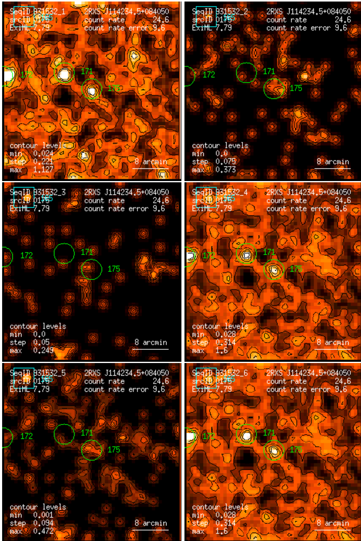
Figure 175: RASS 931532: detection 0175: band rate images, Gaussian filter: (1) PSPC channels 11 – 41, (2) 52 – 90, (3) 91 – 201, (4) 11 – 235, (5) 52 – 201, (6) 11 – 201. Broad band rates in counts/ks. Band rate contour levels in counts/ks/arcmin 2 .
