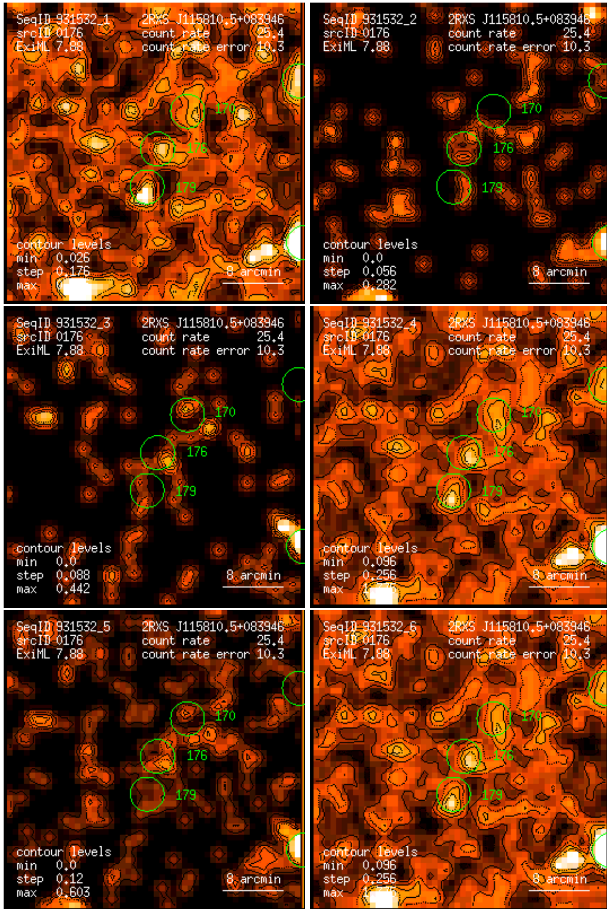
Figure 176: RASS 931532: detection 0176: band rate images, Gaussian filter: (1) PSPC channels 11 – 41, (2) 52 – 90, (3) 91 – 201, (4) 11 – 235, (5) 52 – 201, (6) 11 – 201. Broad band rates in counts/ks. Band rate contour levels in counts/ks/arcmin 2 .
