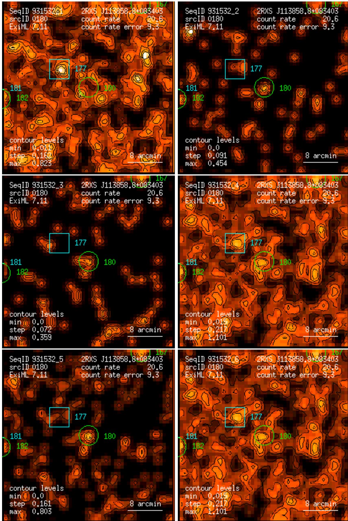
Figure 180: RASS 931532: detection 0180: band rate images, Gaussian filter: (1) PSPC channels 11 – 41, (2) 52 – 90, (3) 91 – 201, (4) 11 – 235, (5) 52 – 201, (6) 11 – 201. Broad band rates in counts/ks. Band rate contour levels in counts/ks/arcmin 2 .
