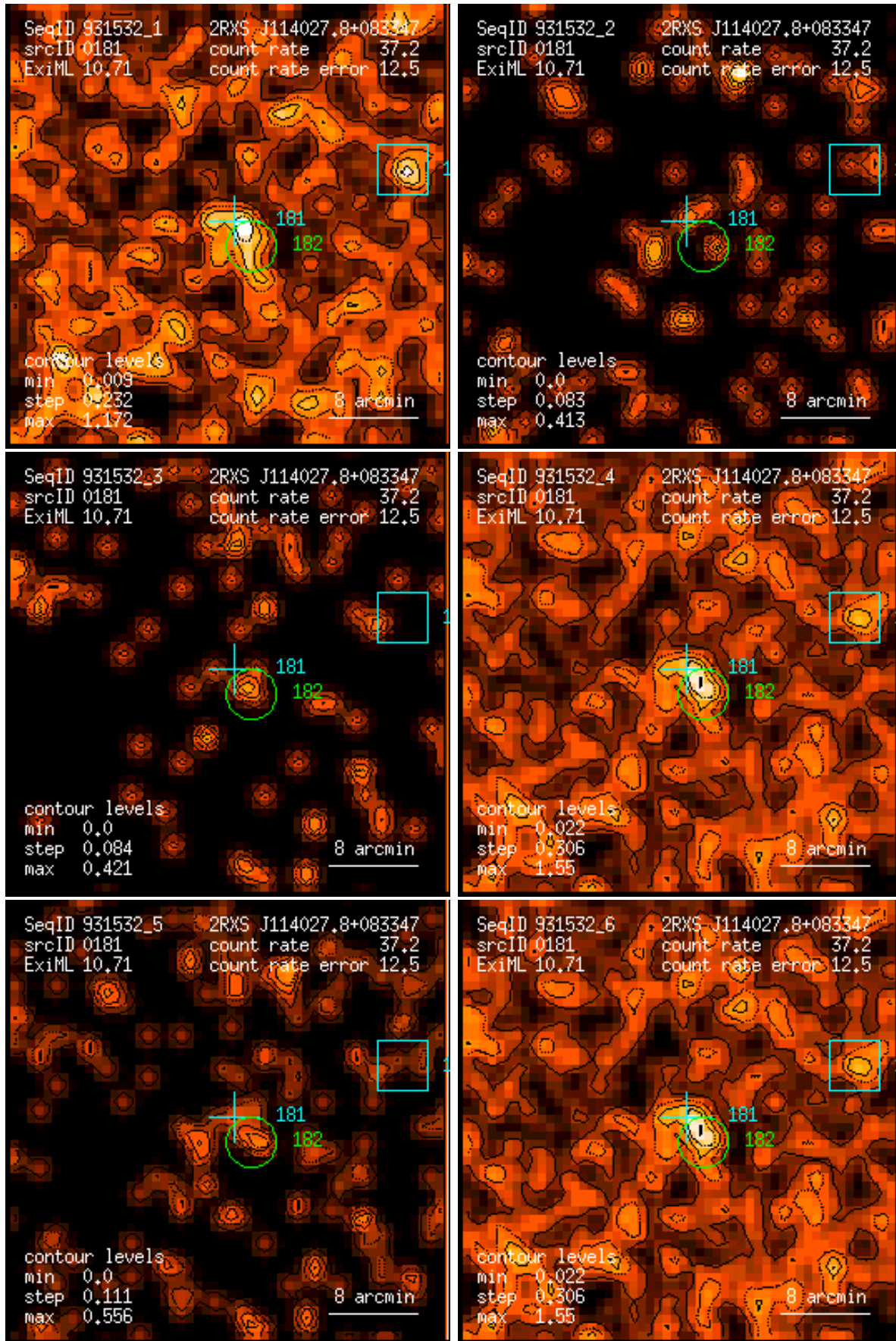
Figure 181: RASS 931532: detection 0181: band rate images, Gaussian filter: (1) PSPC channels 11 – 41, (2) 52 – 90, (3) 91 – 201, (4) 11 – 235, (5) 52 – 201, (6) 11 – 201. Broad band rates in counts/ks. Band rate contour levels in counts/ks/arcmin 2 .
