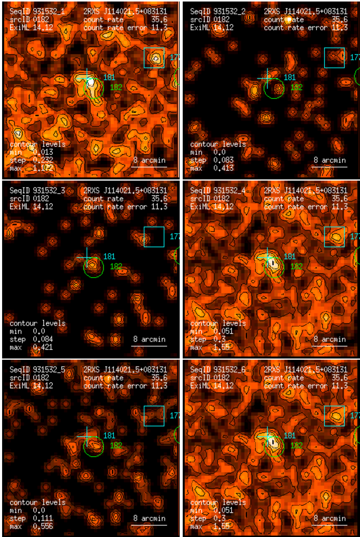
Figure 182: RASS 931532: detection 0182: band rate images, Gaussian filter: (1) PSPC channels 11 – 41, (2) 52 – 90, (3) 91 – 201, (4) 11 – 235, (5) 52 – 201, (6) 11 – 201. Broad band rates in counts/ks. Band rate contour levels in counts/ks/arcmin 2 .
