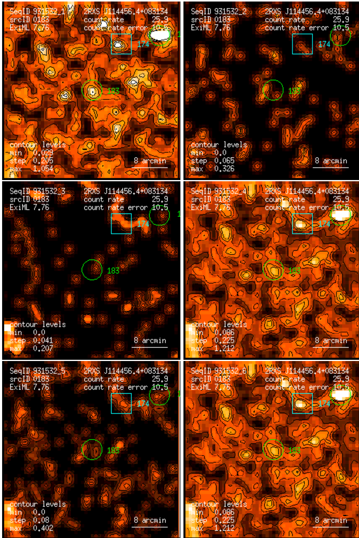
Figure 183: RASS 931532: detection 0183: band rate images, Gaussian filter: (1) PSPC channels 11 – 41, (2) 52 – 90, (3) 91 – 201, (4) 11 – 235, (5) 52 – 201, (6) 11 – 201. Broad band rates in counts/ks. Band rate contour levels in counts/ks/arcmin 2 .
