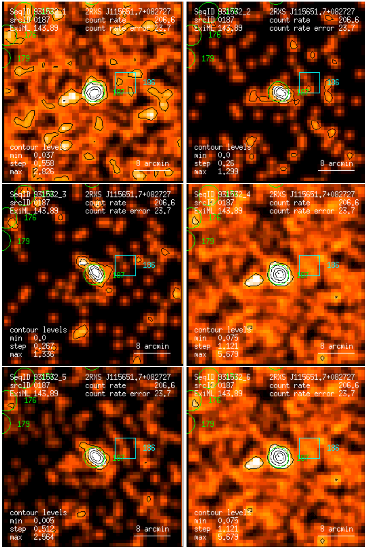
Figure 187: RASS 931532: detection 0187: band rate images, Gaussian filter: (1) PSPC channels 11 – 41, (2) 52 – 90, (3) 91 – 201, (4) 11 – 235, (5) 52 – 201, (6) 11 – 201. Broad band rates in counts/ks. Band rate contour levels in counts/ks/arcmin 2 .
