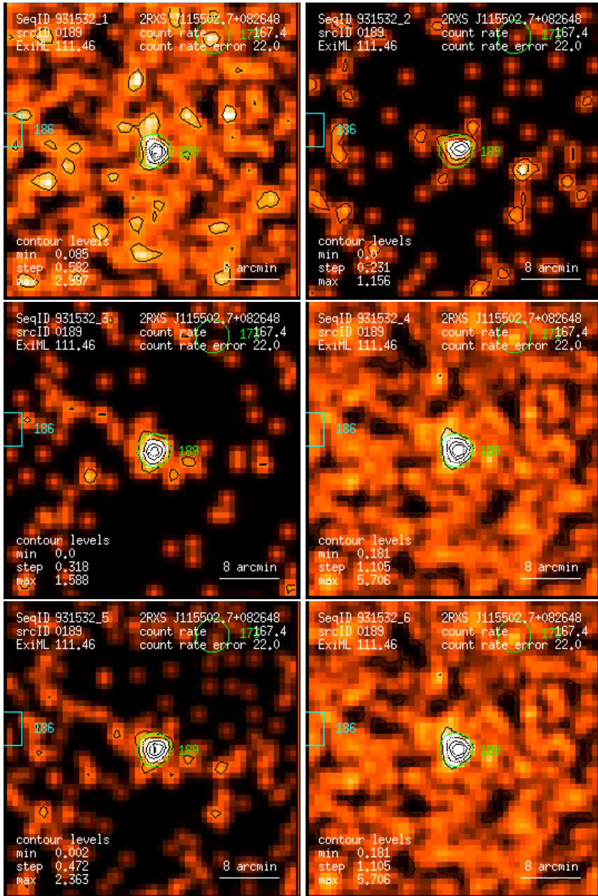
Figure 189: RASS 931532: detection 0189: band rate images, Gaussian filter: (1) PSPC channels 11 – 41, (2) 52 – 90, (3) 91 – 201, (4) 11 – 235, (5) 52 – 201, (6) 11 – 201. Broad band rates in counts/ks. Band rate contour levels in counts/ks/arcmin 2 .
