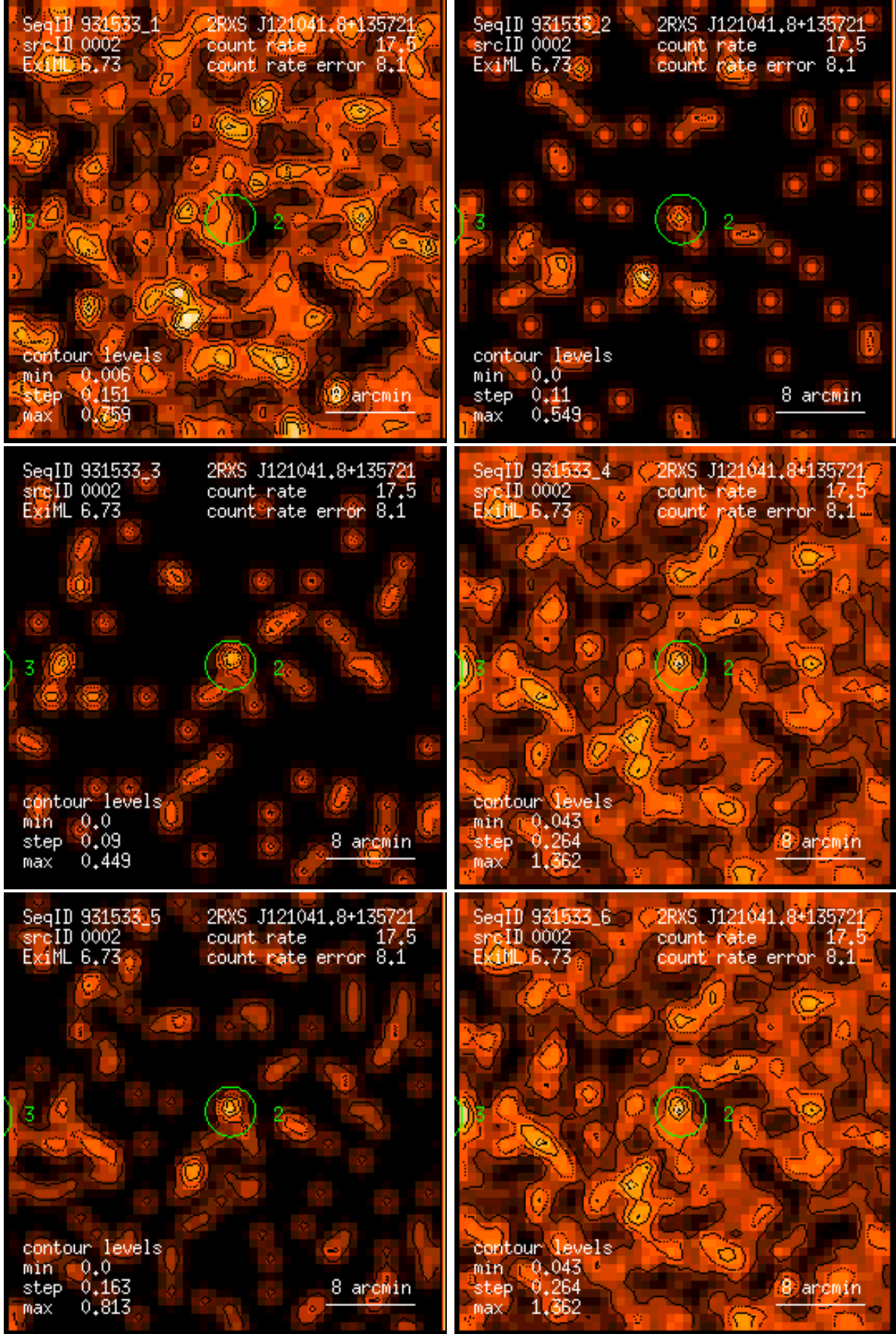
Figure 2: RASS 931533: detection 0002: band rate images, Gaussian filter: (1) PSPC channels 11 – 41, (2) 52 – 90, (3) 91 – 201, (4) 11 – 235, (5) 52 – 201, (6) 11 – 201. Broad band rates in counts/ks. Band rate contour levels in counts/ks/arcmin 2 .
