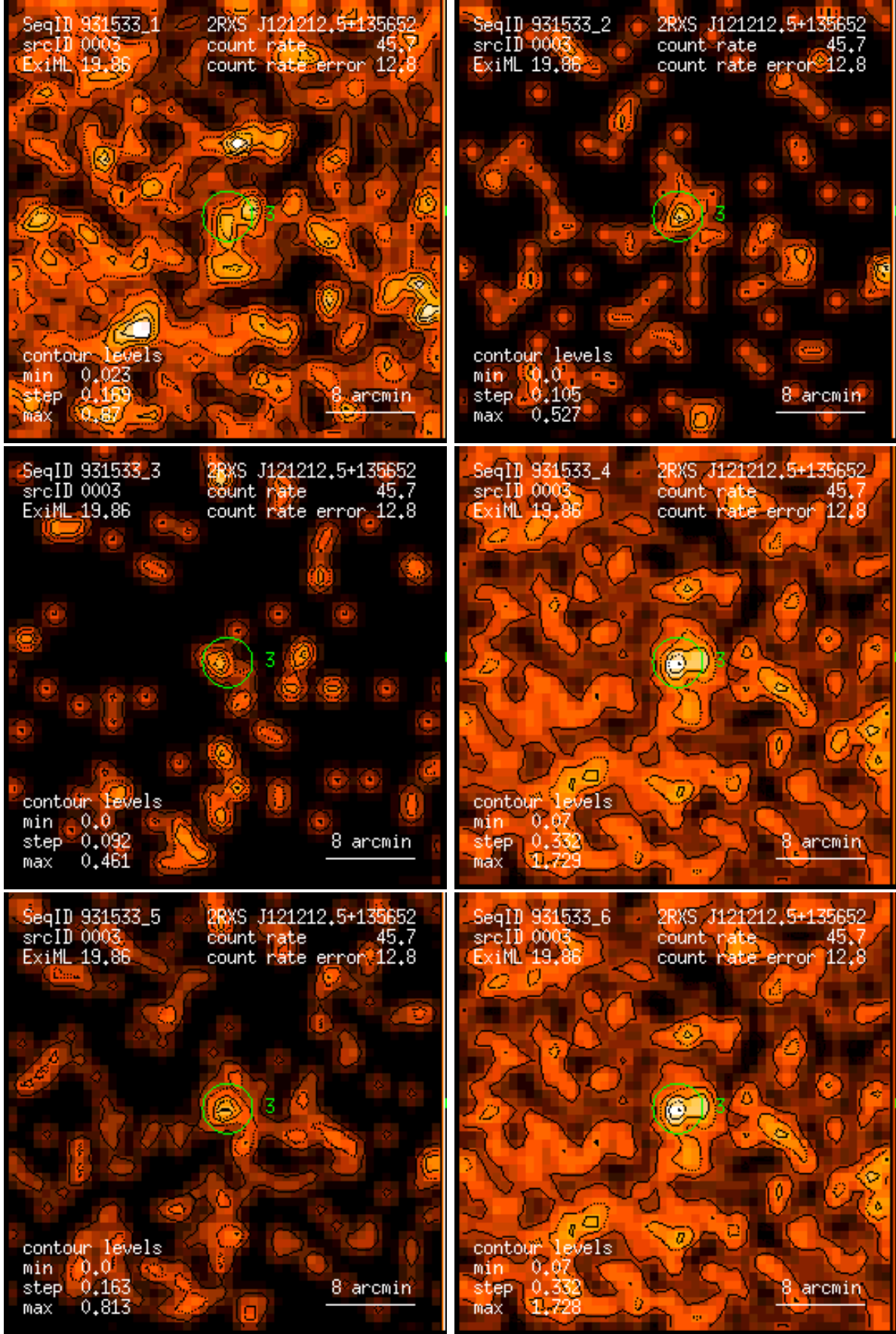
Figure 3: RASS 931533: detection 0003: band rate images, Gaussian filter: (1) PSPC channels 11 – 41, (2) 52 – 90, (3) 91 – 201, (4) 11 – 235, (5) 52 – 201, (6) 11 – 201. Broad band rates in counts/ks. Band rate contour levels in counts/ks/arcmin 2 .
