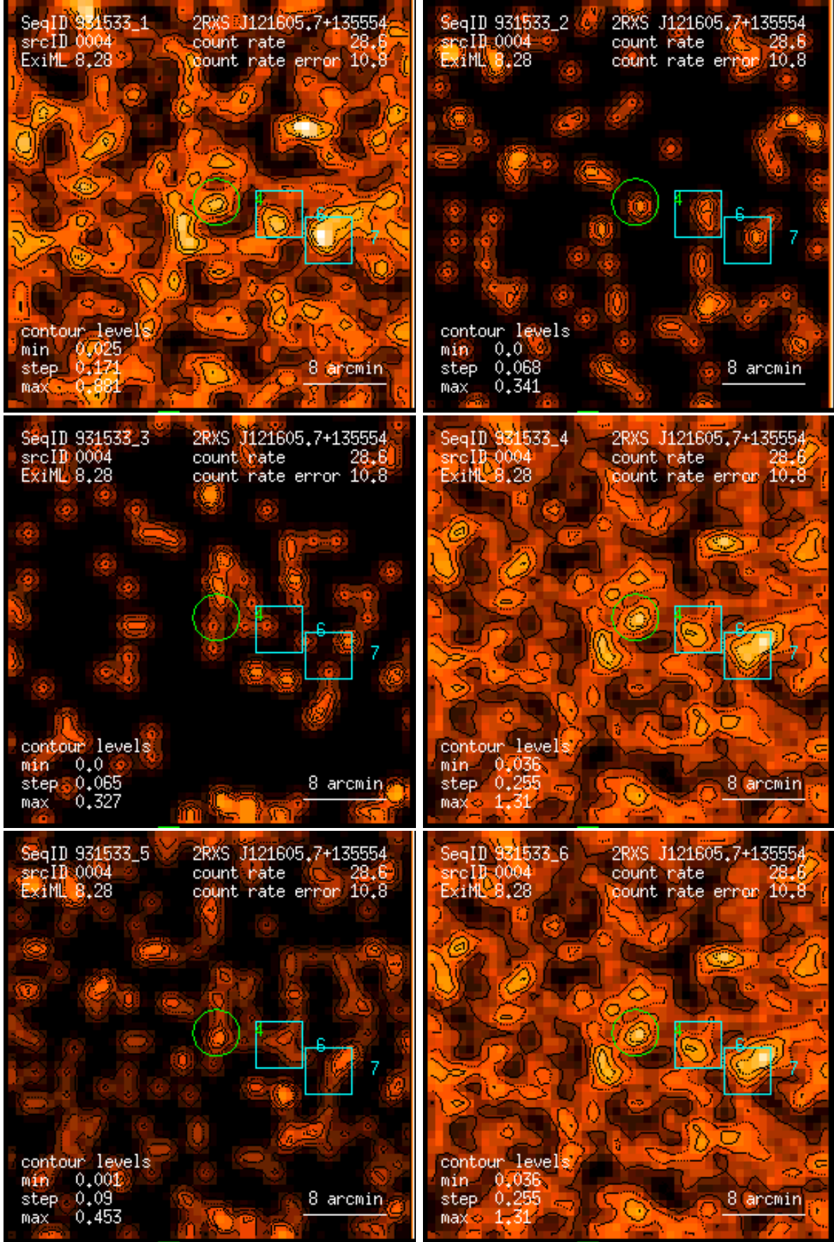
Figure 4: RASS 931533: detection 0004: band rate images, Gaussian filter: (1) PSPC channels 11 – 41, (2) 52 – 90, (3) 91 – 201, (4) 11 – 235, (5) 52 – 201, (6) 11 – 201. Broad band rates in counts/ks. Band rate contour levels in counts/ks/arcmin 2 .
