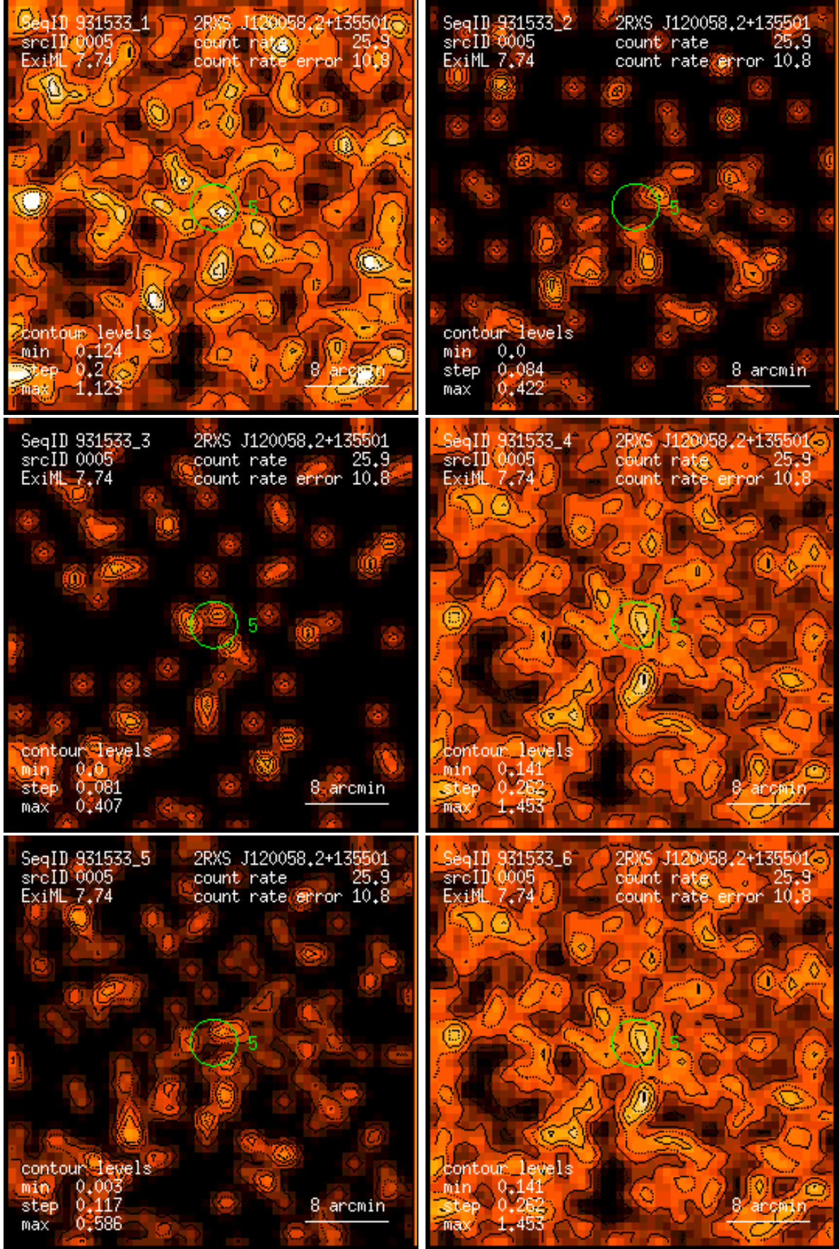
Figure 5: RASS 931533: detection 0005: band rate images, Gaussian filter: (1) PSPC channels 11 – 41, (2) 52 – 90, (3) 91 – 201, (4) 11 – 235, (5) 52 – 201, (6) 11 – 201. Broad band rates in counts/ks. Band rate contour levels in counts/ks/arcmin 2 .
