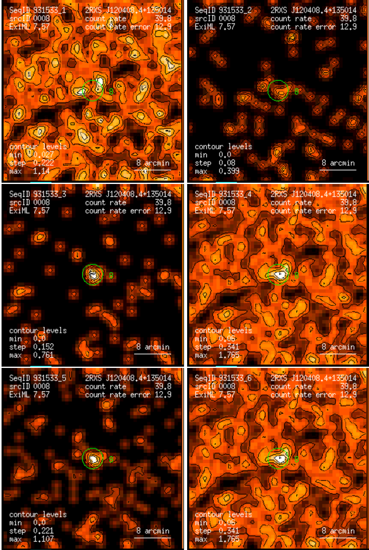
Figure 8: RASS 931533: detection 0008: band rate images, Gaussian filter: (1) PSPC channels 11 – 41, (2) 52 – 90, (3) 91 – 201, (4) 11 – 235, (5) 52 – 201, (6) 11 – 201. Broad band rates in counts/ks. Band rate contour levels in counts/ks/arcmin 2 .
