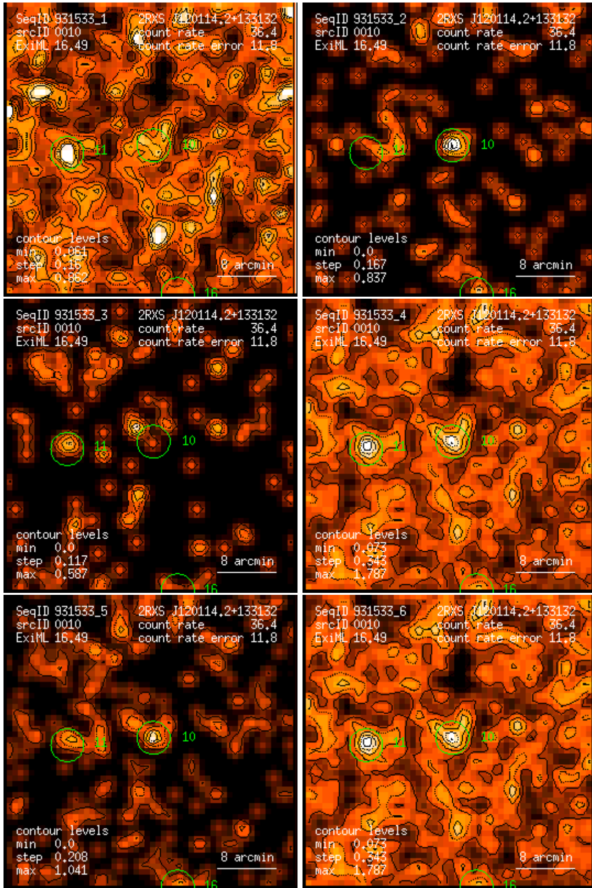
Figure 10: RASS 931533: detection 0010: band rate images, Gaussian filter: (1) PSPC channels 11 – 41, (2) 52 – 90, (3) 91 – 201, (4) 11 – 235, (5) 52 – 201, (6) 11 – 201. Broad band rates in counts/ks. Band rate contour levels in counts/ks/arcmin 2 .
