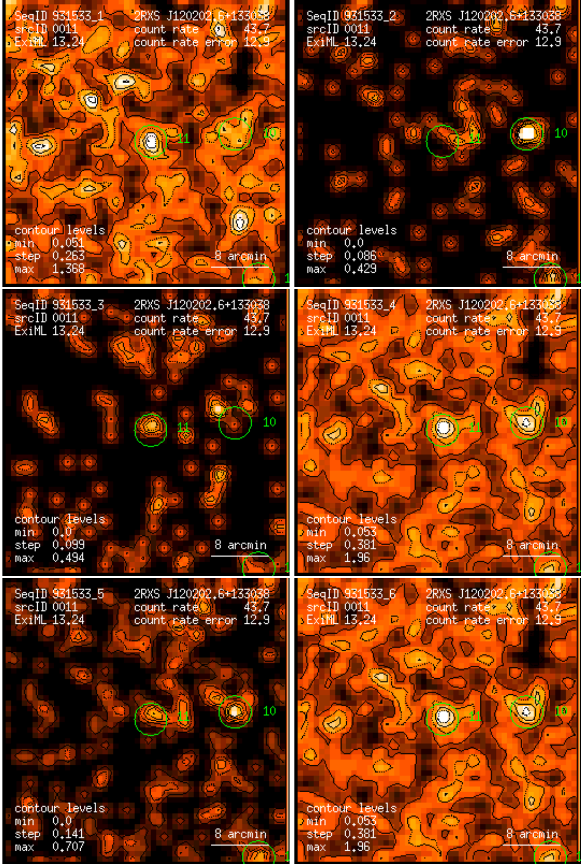
Figure 11: RASS 931533: detection 0011: band rate images, Gaussian filter: (1) PSPC channels 11 – 41, (2) 52 – 90, (3) 91 – 201, (4) 11 – 235, (5) 52 – 201, (6) 11 – 201. Broad band rates in counts/ks. Band rate contour levels in counts/ks/arcmin 2 .
