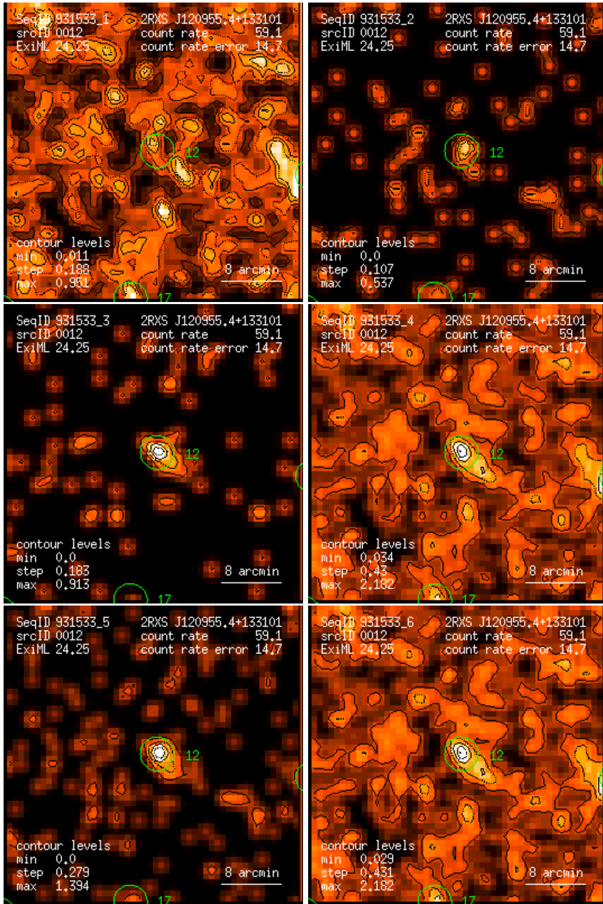
Figure 12: RASS 931533: detection 0012: band rate images, Gaussian filter: (1) PSPC channels 11 – 41, (2) 52 – 90, (3) 91 – 201, (4) 11 – 235, (5) 52 – 201, (6) 11 – 201. Broad band rates in counts/ks. Band rate contour levels in counts/ks/arcmin 2 .
