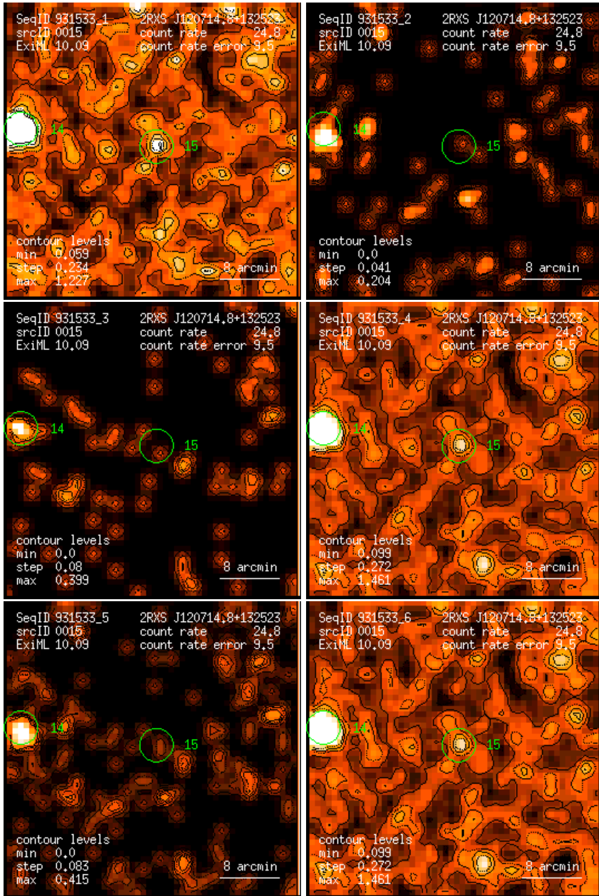
Figure 15: RASS 931533: detection 0015: band rate images, Gaussian filter: (1) PSPC channels 11 – 41, (2) 52 – 90, (3) 91 – 201, (4) 11 – 235, (5) 52 – 201, (6) 11 – 201. Broad band rates in counts/ks. Band rate contour levels in counts/ks/arcmin 2 .
