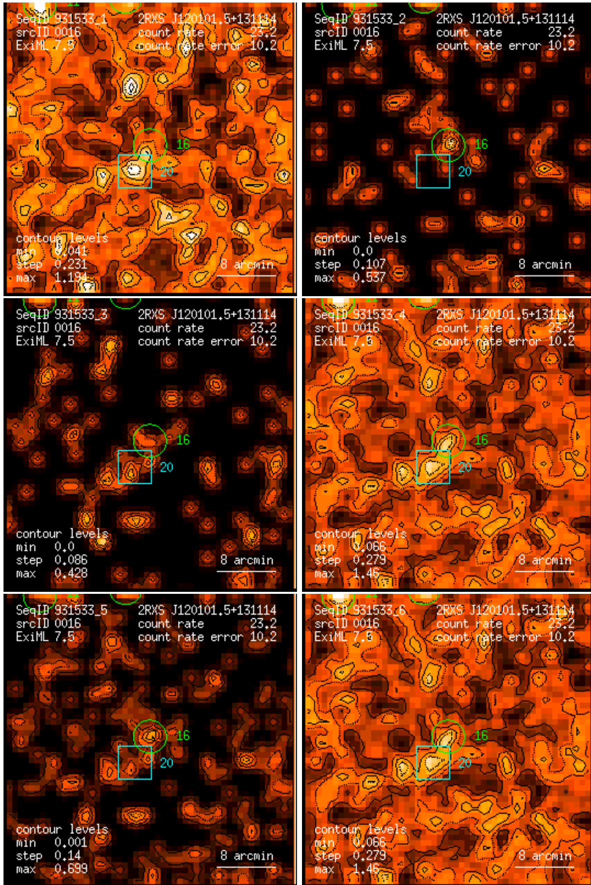
Figure 16: RASS 931533: detection 0016: band rate images, Gaussian filter: (1) PSPC channels 11 – 41, (2) 52 – 90, (3) 91 – 201, (4) 11 – 235, (5) 52 – 201, (6) 11 – 201. Broad band rates in counts/ks. Band rate contour levels in counts/ks/arcmin 2 .
