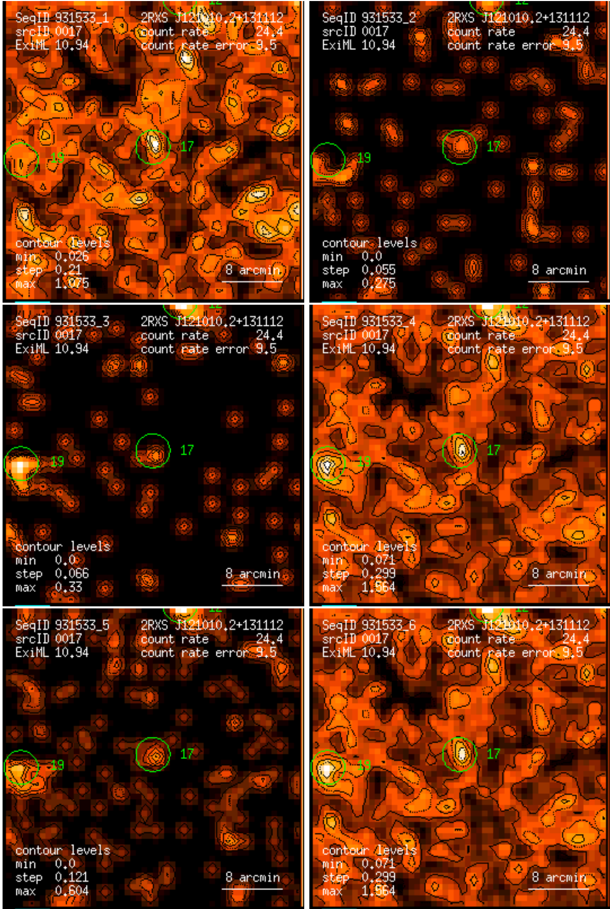
Figure 17: RASS 931533: detection 0017: band rate images, Gaussian filter: (1) PSPC channels 11 – 41, (2) 52 – 90, (3) 91 – 201, (4) 11 – 235, (5) 52 – 201, (6) 11 – 201. Broad band rates in counts/ks. Band rate contour levels in counts/ks/arcmin 2 .
