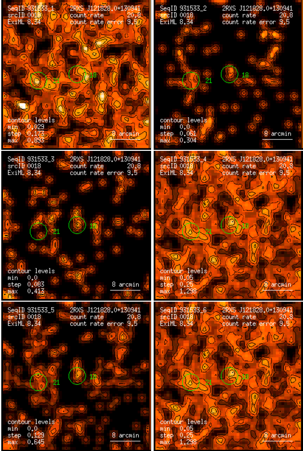
Figure 18: RASS 931533: detection 0018: band rate images, Gaussian filter: (1) PSPC channels 11 – 41, (2) 52 – 90, (3) 91 – 201, (4) 11 – 235, (5) 52 – 201, (6) 11 – 201. Broad band rates in counts/ks. Band rate contour levels in counts/ks/arcmin 2 .
