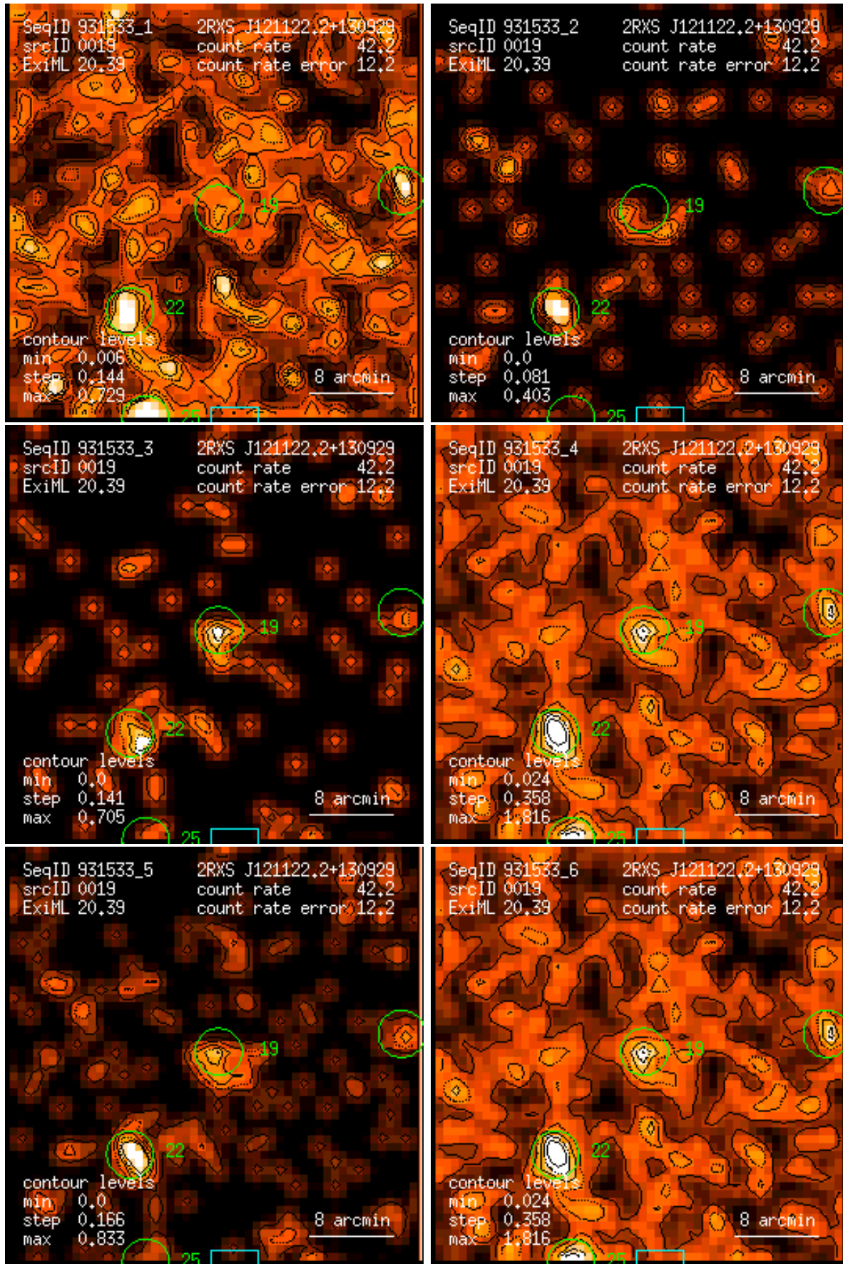
Figure 19: RASS 931533: detection 0019: band rate images, Gaussian filter: (1) PSPC channels 11 – 41, (2) 52 – 90, (3) 91 – 201, (4) 11 – 235, (5) 52 – 201, (6) 11 – 201. Broad band rates in counts/ks. Band rate contour levels in counts/ks/arcmin 2 .
