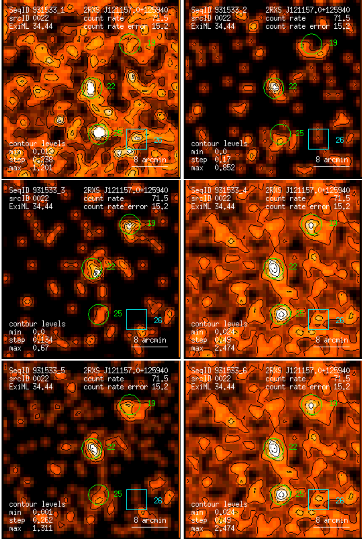
Figure 22: RASS 931533: detection 0022: band rate images, Gaussian filter: (1) PSPC channels 11 – 41, (2) 52 – 90, (3) 91 – 201, (4) 11 – 235, (5) 52 – 201, (6) 11 – 201. Broad band rates in counts/ks. Band rate contour levels in counts/ks/arcmin 2 .
