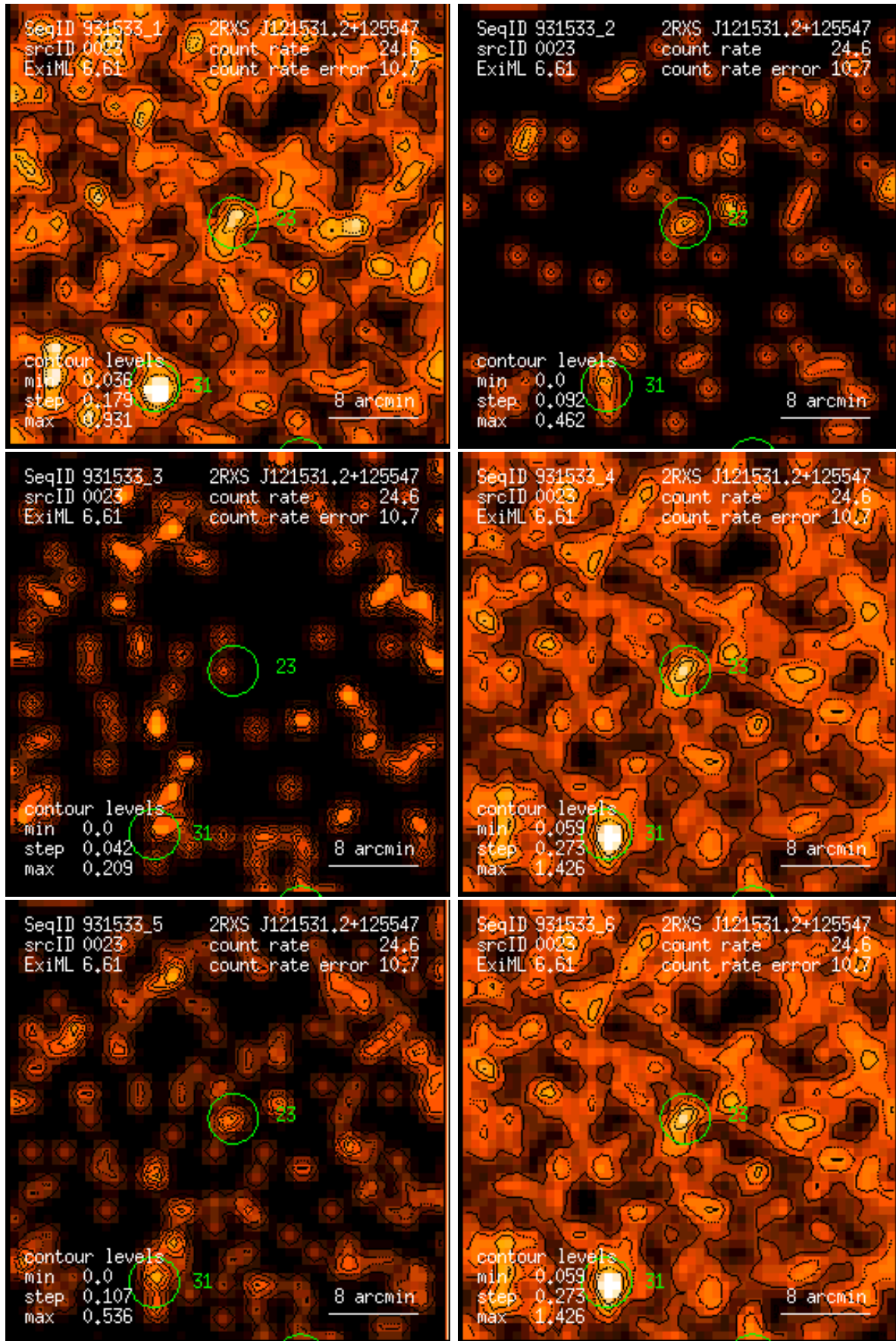
Figure 23: RASS 931533: detection 0023: band rate images, Gaussian filter: (1) PSPC channels 11 – 41, (2) 52 – 90, (3) 91 – 201, (4) 11 – 235, (5) 52 – 201, (6) 11 – 201. Broad band rates in counts/ks. Band rate contour levels in counts/ks/arcmin 2 .
