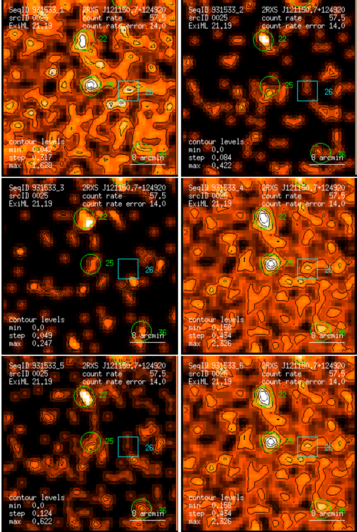
Figure 25: RASS 931533: detection 0025: band rate images, Gaussian filter: (1) PSPC channels 11 – 41, (2) 52 – 90, (3) 91 – 201, (4) 11 – 235, (5) 52 – 201, (6) 11 – 201. Broad band rates in counts/ks. Band rate contour levels in counts/ks/arcmin 2 .
