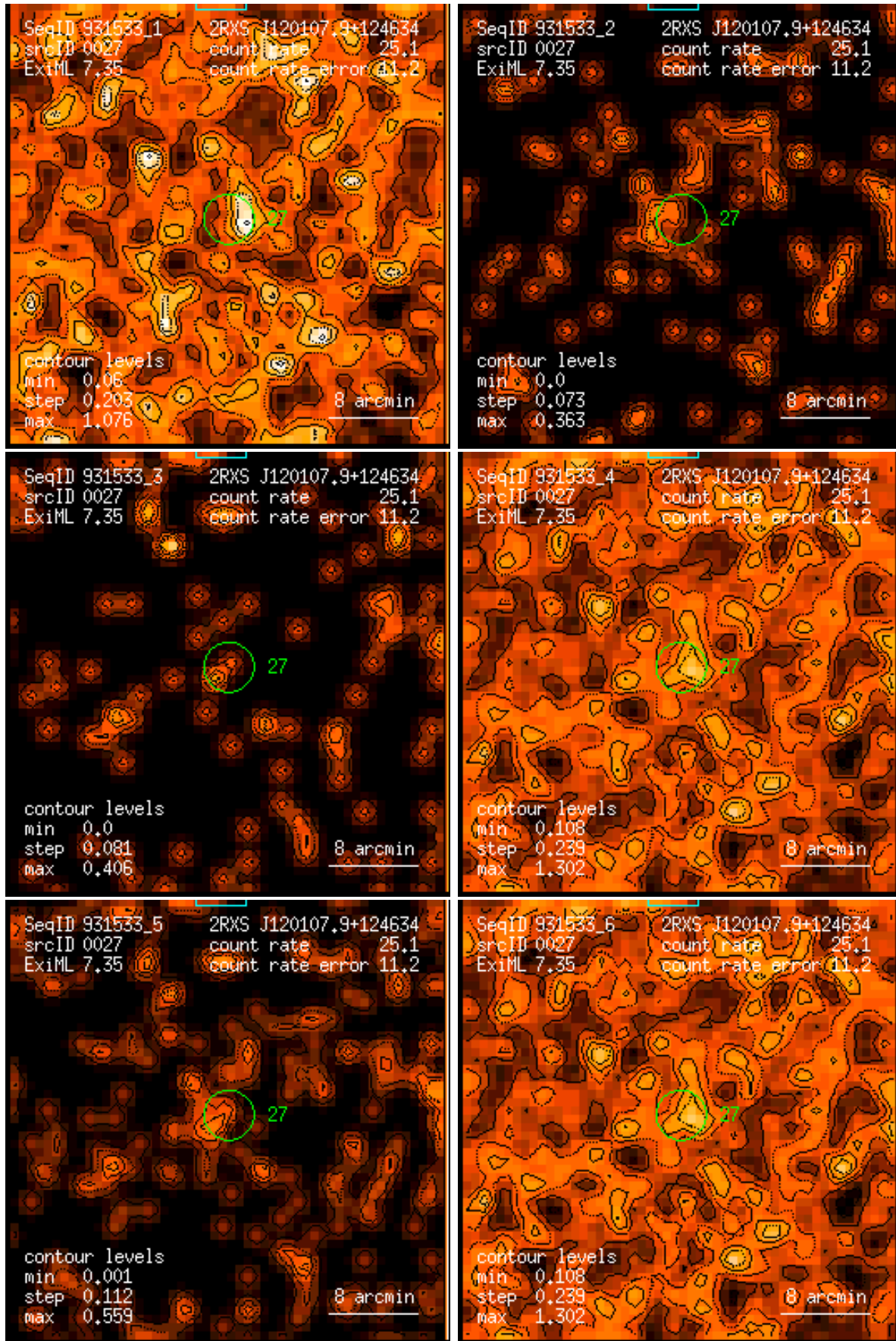
Figure 27: RASS 931533: detection 0027: band rate images, Gaussian filter: (1) PSPC channels 11 – 41, (2) 52 – 90, (3) 91 – 201, (4) 11 – 235, (5) 52 – 201, (6) 11 – 201. Broad band rates in counts/ks. Band rate contour levels in counts/ks/arcmin 2 .
