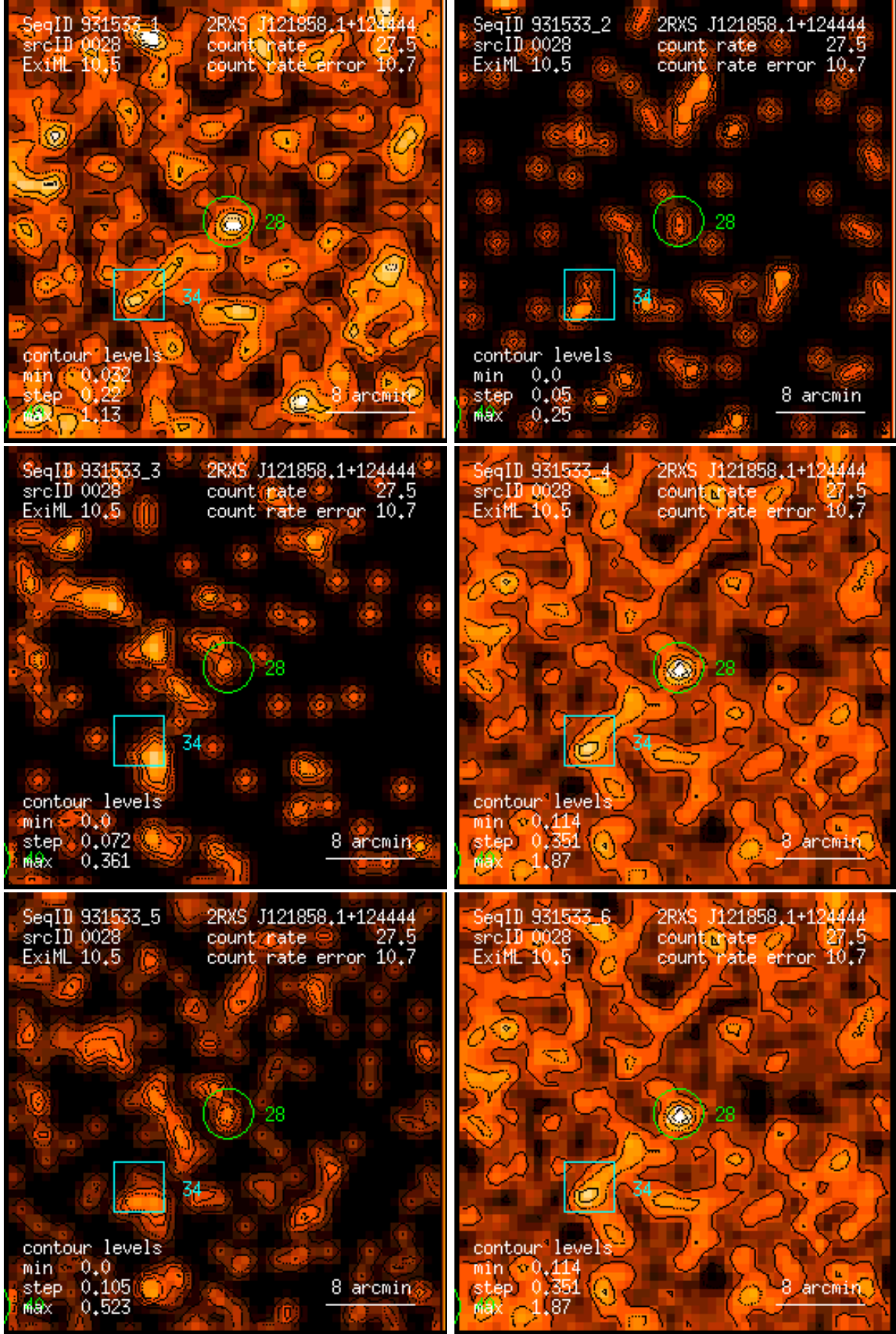
Figure 28: RASS 931533: detection 0028: band rate images, Gaussian filter: (1) PSPC channels 11 – 41, (2) 52 – 90, (3) 91 – 201, (4) 11 – 235, (5) 52 – 201, (6) 11 – 201. Broad band rates in counts/ks. Band rate contour levels in counts/ks/arcmin 2 .
