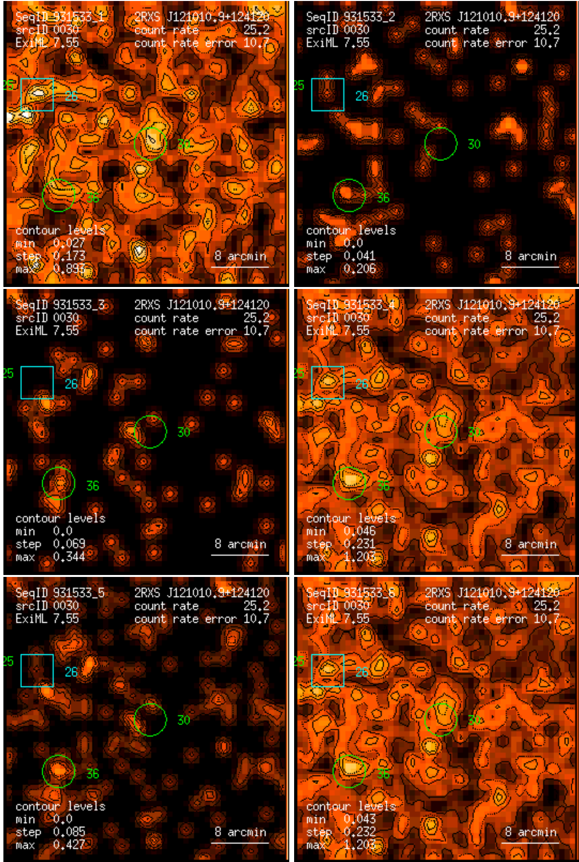
Figure 30: RASS 931533: detection 0030: band rate images, Gaussian filter: (1) PSPC channels 11 – 41, (2) 52 – 90, (3) 91 – 201, (4) 11 – 235, (5) 52 – 201, (6) 11 – 201. Broad band rates in counts/ks. Band rate contour levels in counts/ks/arcmin 2 .
