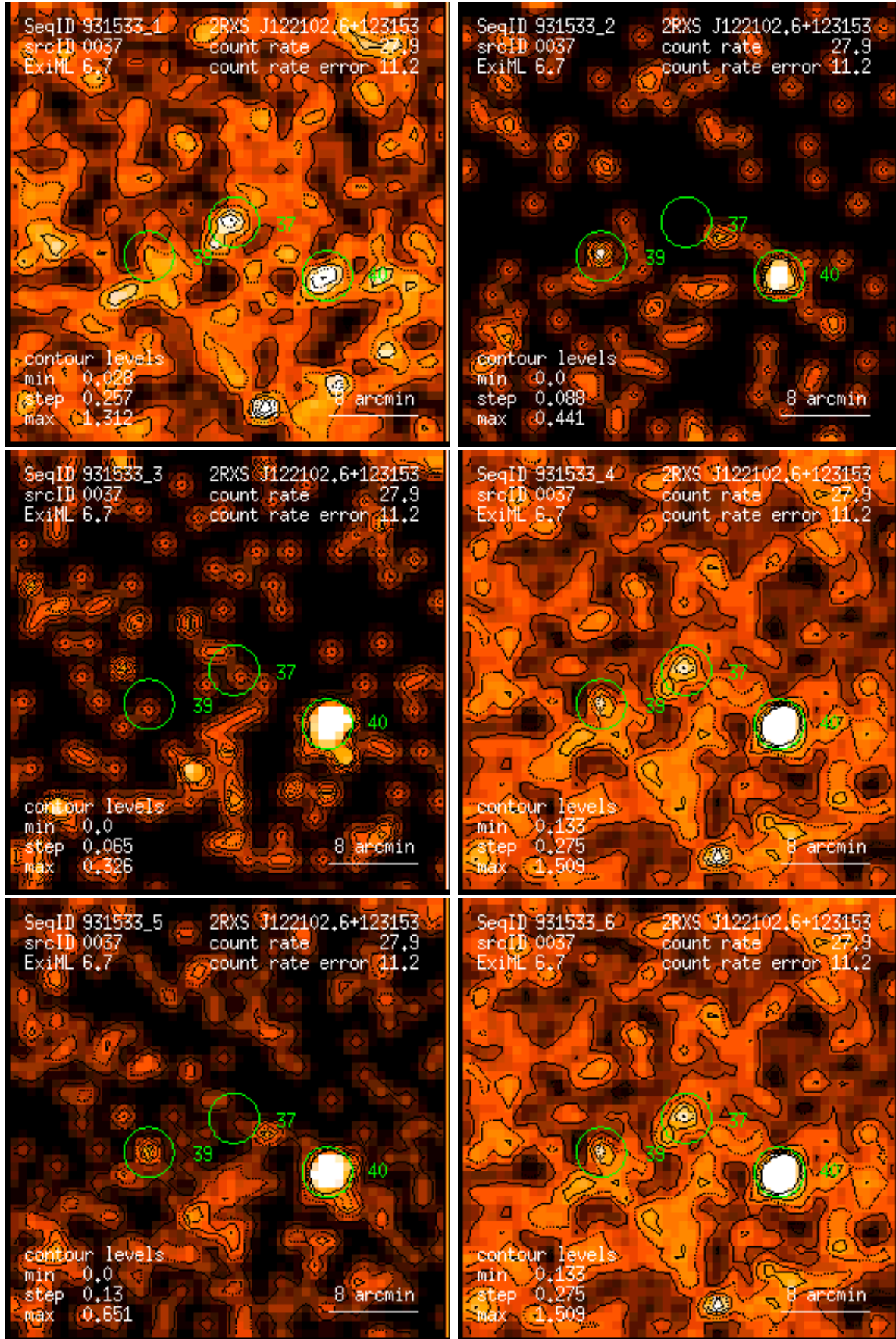
Figure 37: RASS 931533: detection 0037: band rate images, Gaussian filter: (1) PSPC channels 11 – 41, (2) 52 – 90, (3) 91 – 201, (4) 11 – 235, (5) 52 – 201, (6) 11 – 201. Broad band rates in counts/ks. Band rate contour levels in counts/ks/arcmin 2 .
