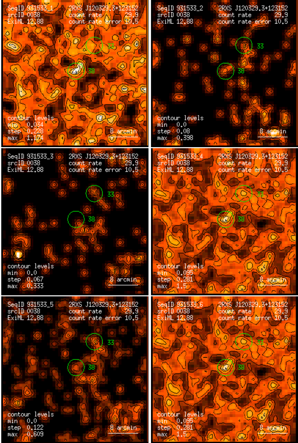
Figure 38: RASS 931533: detection 0038: band rate images, Gaussian filter: (1) PSPC channels 11 – 41, (2) 52 – 90, (3) 91 – 201, (4) 11 – 235, (5) 52 – 201, (6) 11 – 201. Broad band rates in counts/ks. Band rate contour levels in counts/ks/arcmin 2 .
